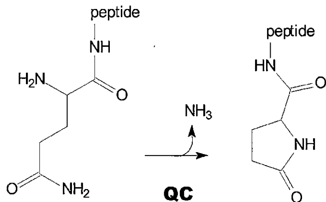
Scheme 1: Cyclization of glutamine by QC
