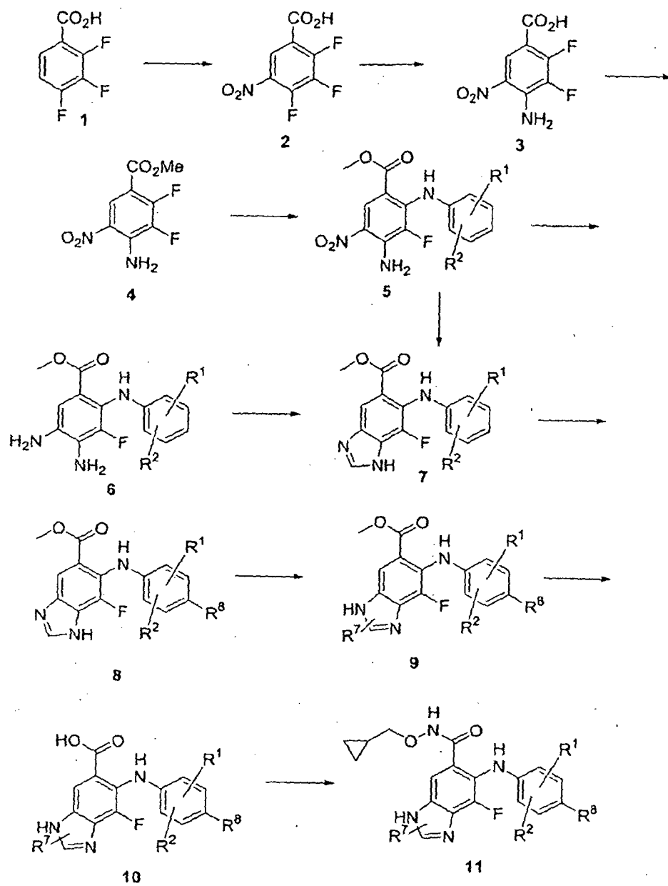
Scheme 1
