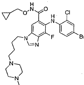
6-(4-Bromo-2-chloro-phenylamino)-7-fluoro-3-[4-(4-methyl-piperazin-1-yl)-butyl]-3H-benzimidazole-5-carboxylic acid cyclopropylmethoxy-amide (18dd)
