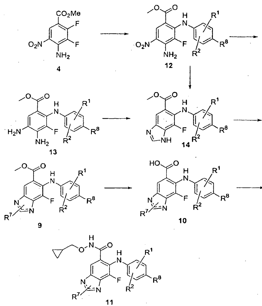
Scheme 2
