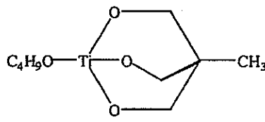
1-(1-Butoxy)-4-methyl-2,6,7-trioxabicyclo[2,2,2]octane
