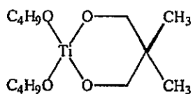
Di-1-butyl 2,2-dimethylpropane-1,3-dioxytitanate
