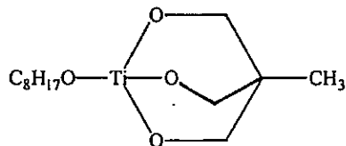
1-(2-ethyl-1-hexoxy)-4-methyl-2,6,7-trioxabicyclo[2,2,2]octane
