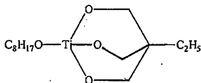
1-(2-ethyl-1-hexoxy)-4-ethyl-2,6,7-trioxabicyclo[2,2,2]octane
