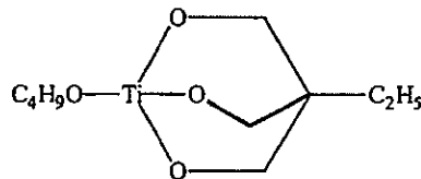
1-(1-Butoxy)-4-ethyl-2,6,7-trioxabicyclo[2,2,2]octane
