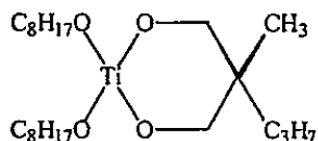
Di(2-ethyl-1-hexyl) 2-(1-propyl)-2-methylpropane-1,3-dioxytitanate
