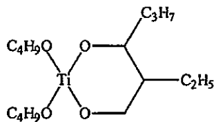
Di-1-butyl 2-ethylhexane-1,3-dioxytitanate
