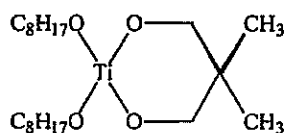
Di(2-ethyl-1-hexyl) 2,2-dimethylpropane-1,3-dioxytitanate
