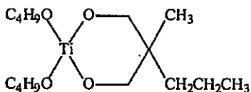
Di-1-butyl 2-(1-propyl)-2-methylpropane-1,3-dioxytitanate
