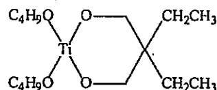
Di-1-butyl 2,2-diethylpropane-1,3-dioxytitanate
