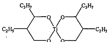
Bis(2-ethyl-1,3-hexylene) titanate
