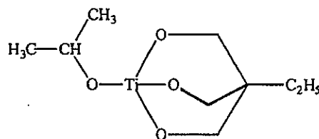
1-(2-Propoxy)-4-ethyl-2,6,7-trioxabicyclo[2,2,2]octane
