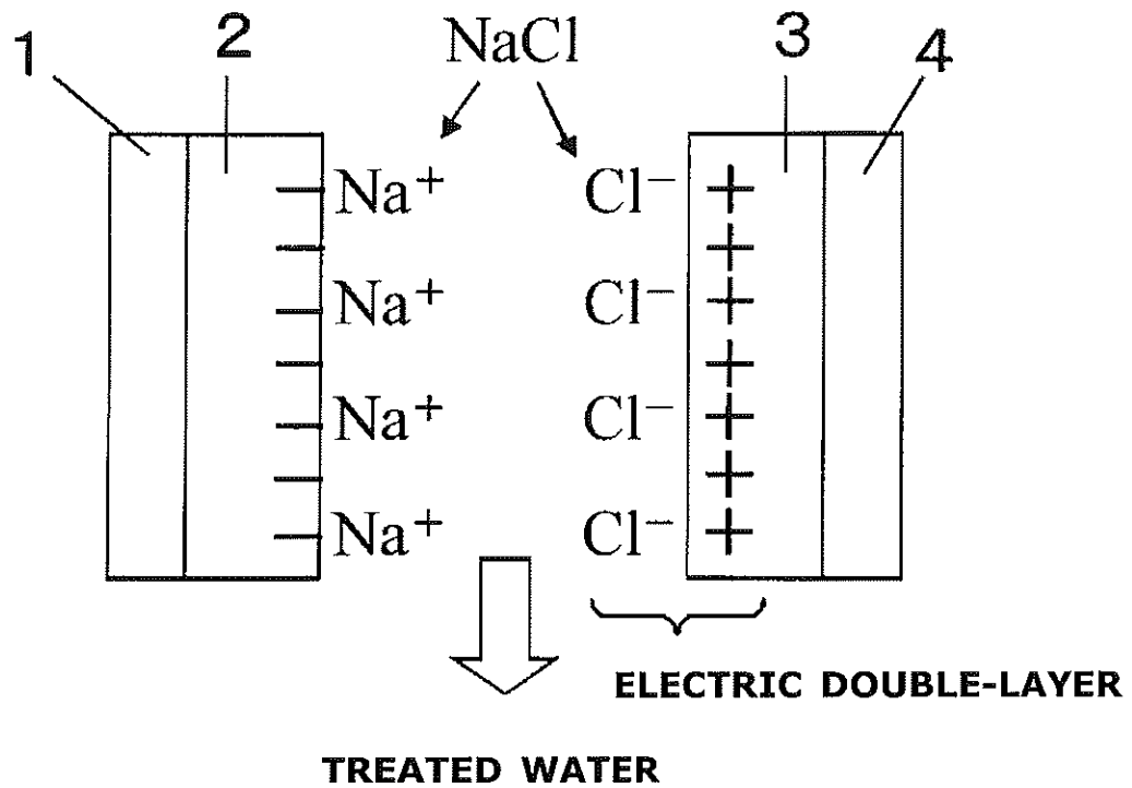
Fig.1 [VOLTAGE APPLICATION STEP: DESALTING]
