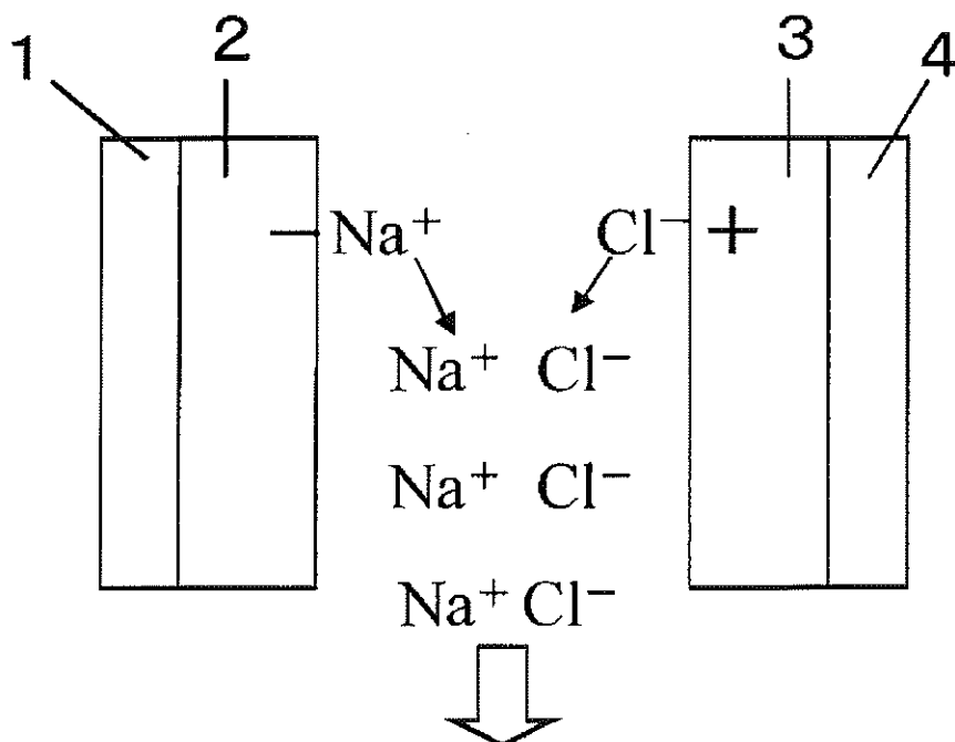
Fig.2 [SHORT-CIRCUITING STEP: DRAINING]
