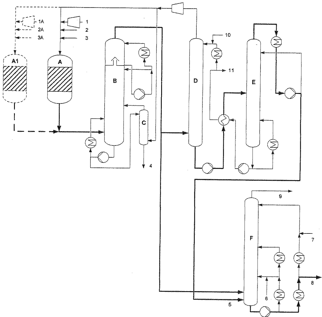
Figure 1: Process option 1
