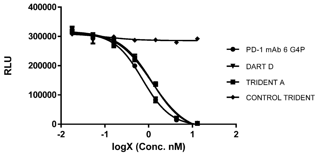
Inhibition of PD-L1 Binding with Immobilized PD-1 and CTLA-4 (1:1 ratio)
