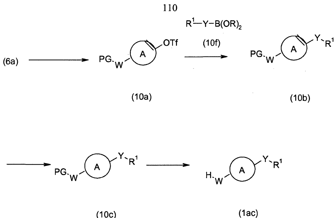
Scheme 10
