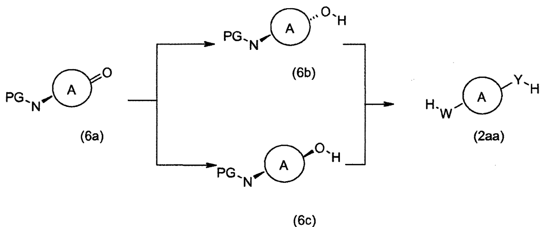
Scheme 6
