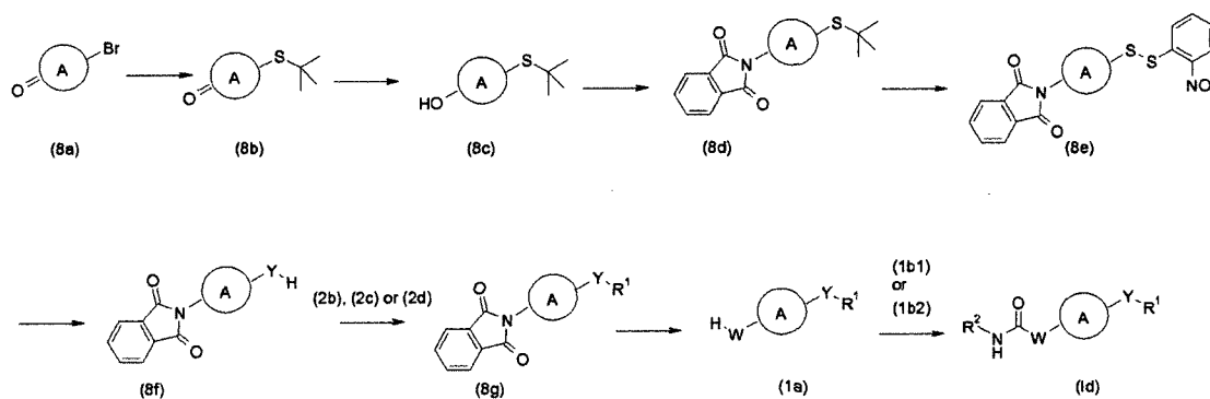
Scheme 8
