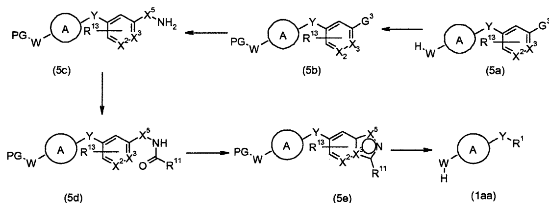
Scheme 5
