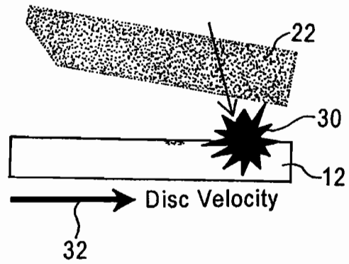
FIG. 2c (PRIOR ART)
