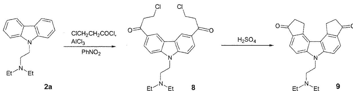
Scheme 5
