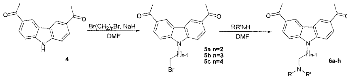
Scheme 3
