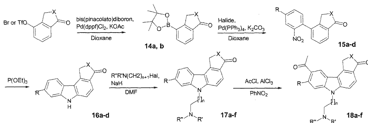
Scheme 7
