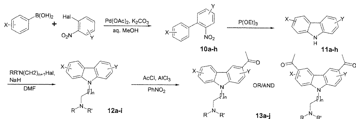
Scheme 6
