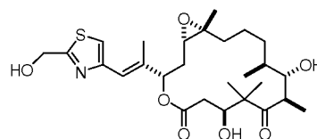
Compound BB
