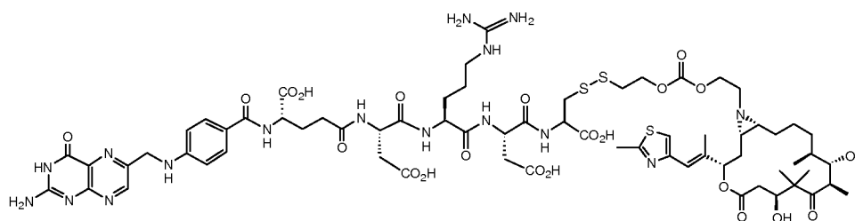
Compound J
