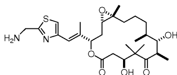
Compound AA
