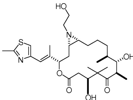
Compound G
