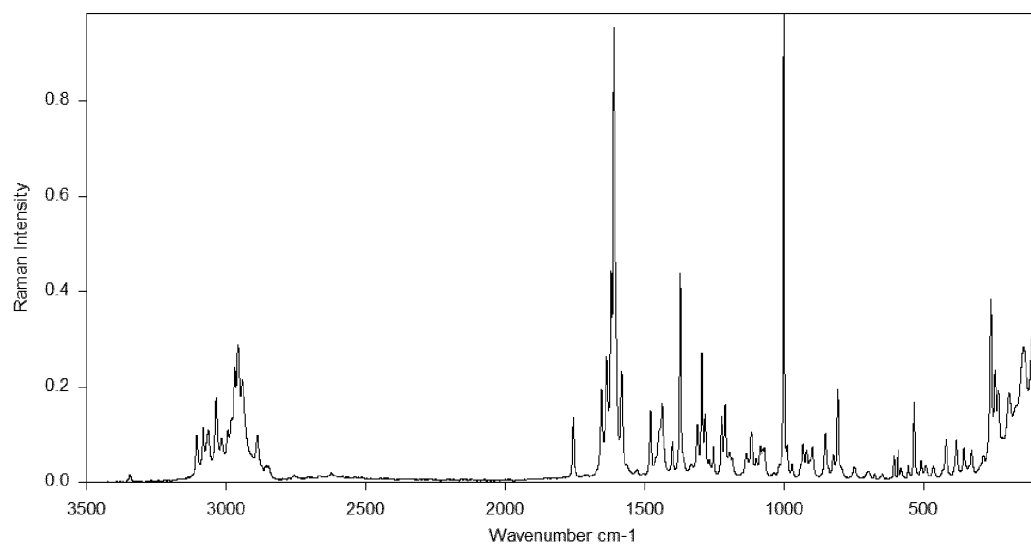
Figure 3: Raman spectrum of the crystal form of compound of formula (Ia)
