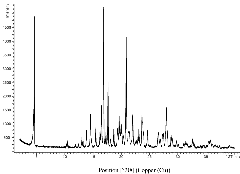
Figure 2: X-ray powder diffractogram of the crystal form of compound of formula (Ib)
