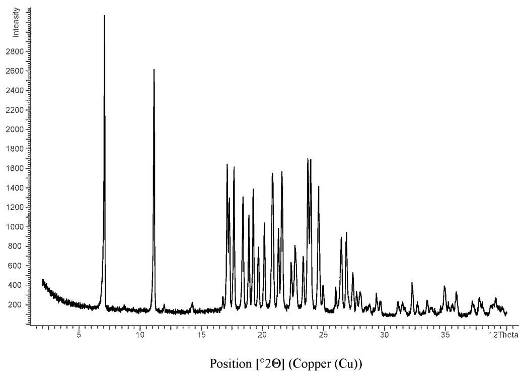
Figure 1: X-ray powder diffractogram of the crystal form of compound of formula (Ia)
