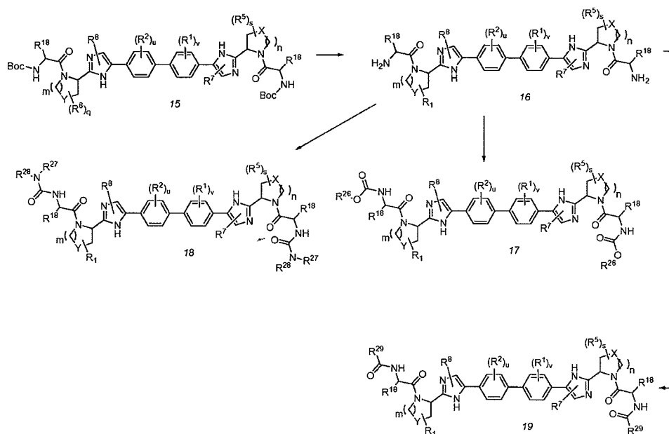
Scheme 4: Symmetric Biphenyls
