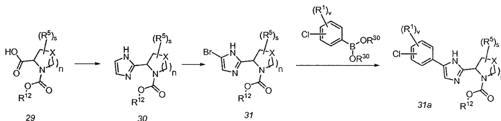
Scheme 7: Heteroaryls
