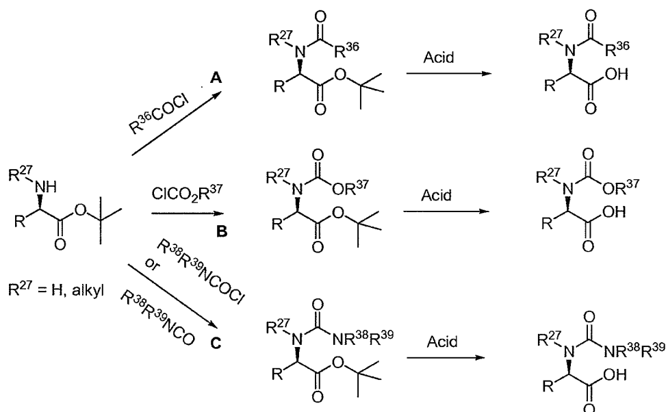
Scheme 13
