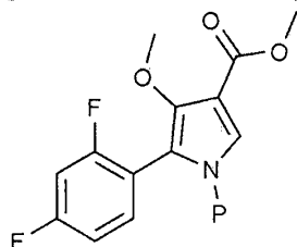
[Chemical Formula 1-6]
