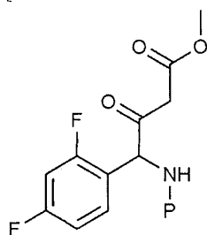
[Chemical Formula 1-5]
