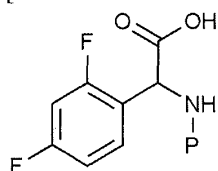
[Chemical Formula 1-4]
