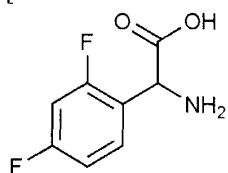
[Chemical Formula 1-3]
