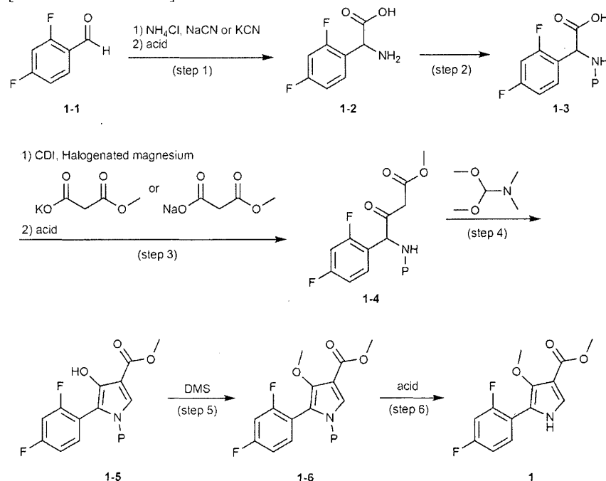
[Reaction Scheme 1]
