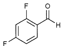
[Chemical Formula 1-2]
