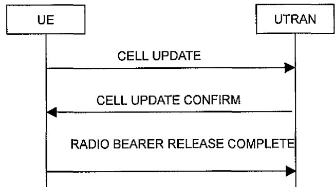
Figure 8.3.1-5: Cell update procedure with radio bearer release
