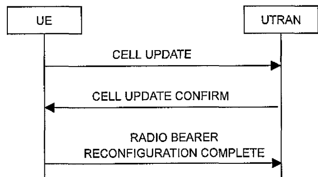
Figure 8.3.1-6: Cell update procedure with radio bearer reconfiguration
