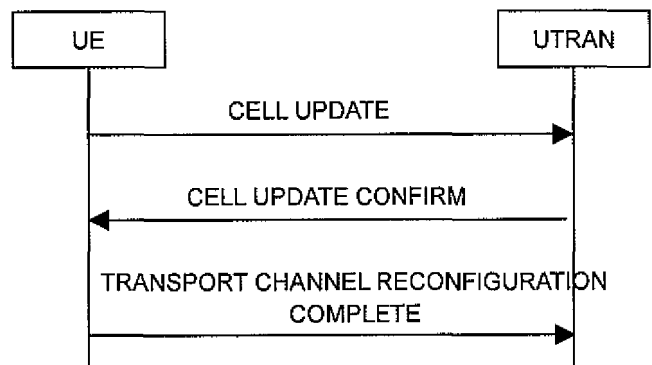
Figure 8.3.1-4: Cell update procedure with transport channel reconfiguration
