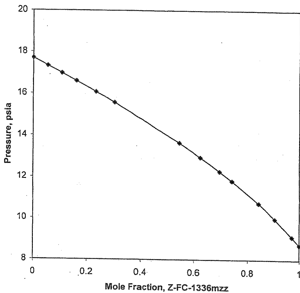
Figure 6. Z-FC-1336mzz and HFC-245fa at 20 C
