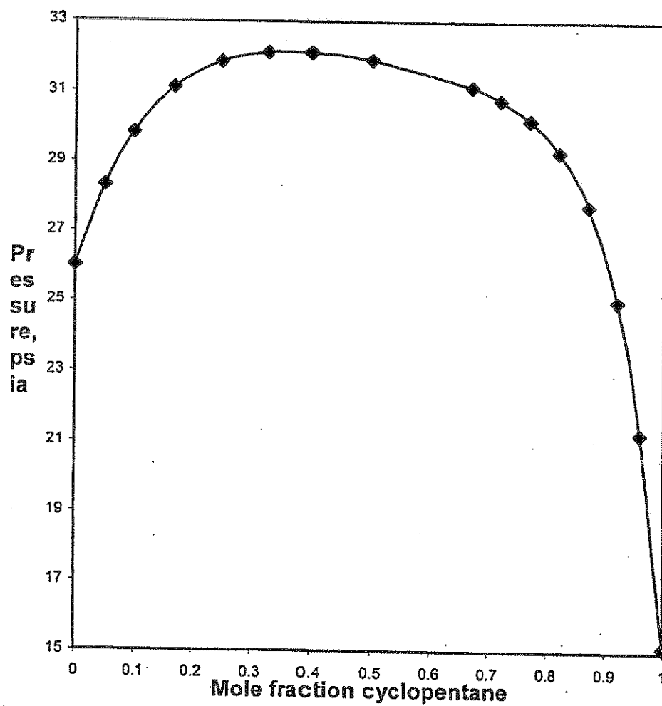
FIG. 8 - Z-FC-1336mzz and Cyclopentane at 50 C
