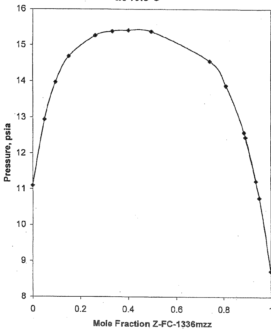
FIGURE 3. Z-FC-1336mzz and Isopentane at 19.9 C
