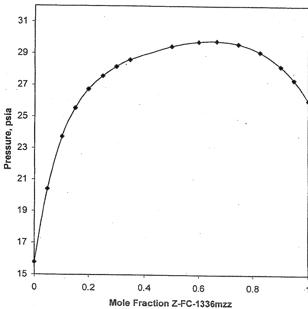
FIGURE 5. Z-FC-1336mzz and trans-1,2-Dichloroethylene at 50.07 C
