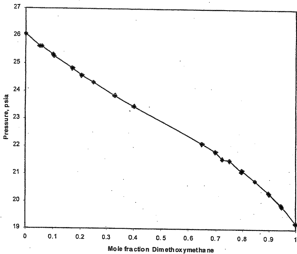
FIGURE 7. Z-FC-1336mzz and Dimethoxymethane at 49.99 C
