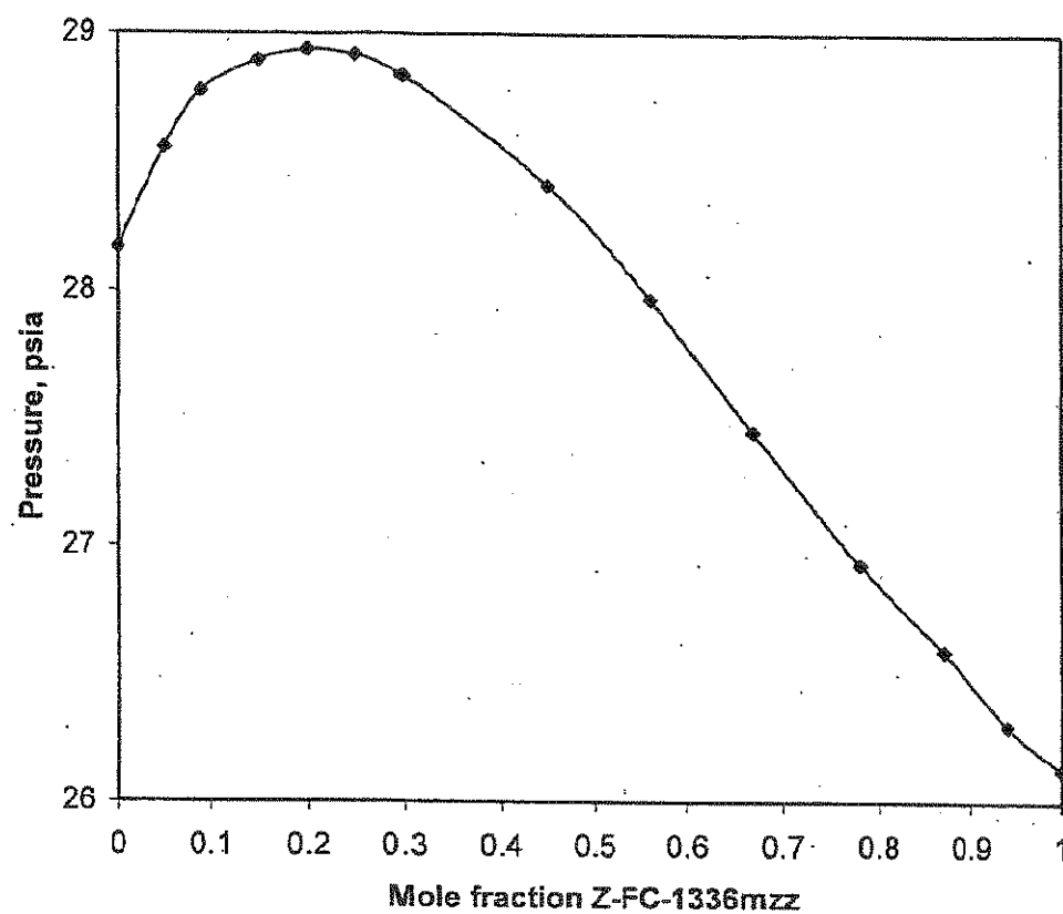
FIGURE 1. VLE DATA for Z-FC-1336mzz/Methyl Formate at 50.1 C
