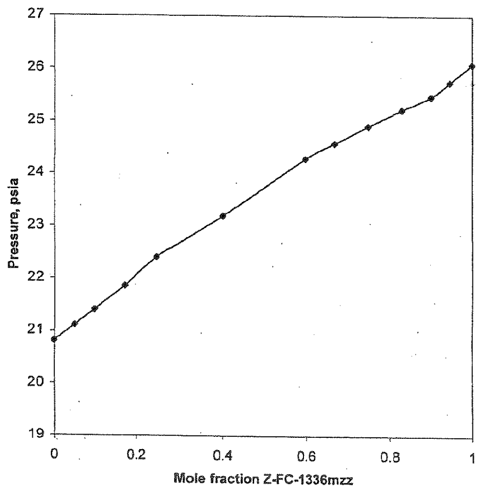
FIG. 4 - Z-FC-1336mzz and HFC-365mfc at 50.1 C
