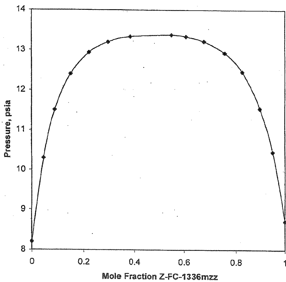
FIGURE 2. Z-FC-1336mzz and n-Pentane at 19.9 C
