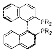
(S)-BINAP
