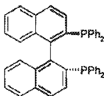
(R)-(+)-BINAP:
