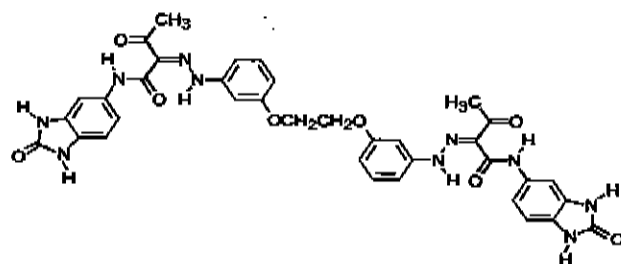
Structural Formula (2)
