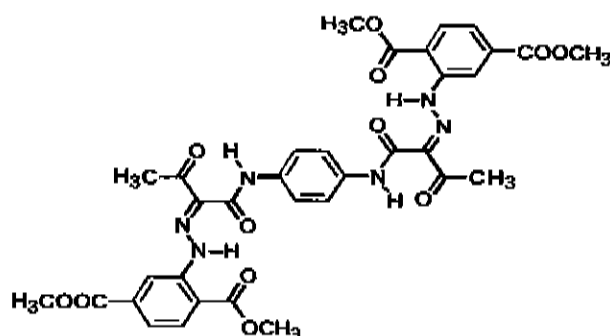
Structural Formula (3)
