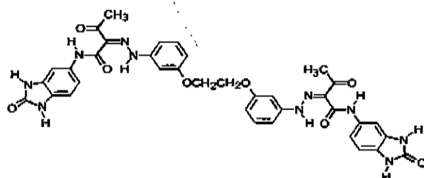
Structural Formula (2)
