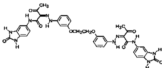
Structural Formula (2)
