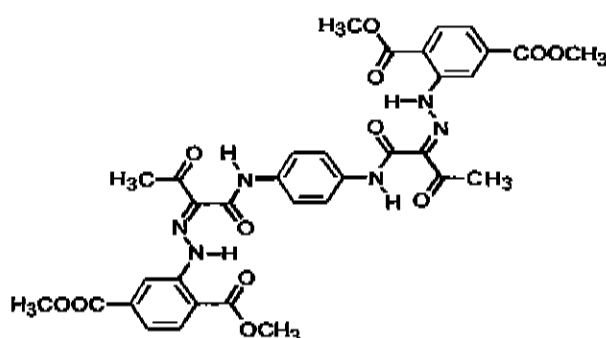
Structural Formula (3)
