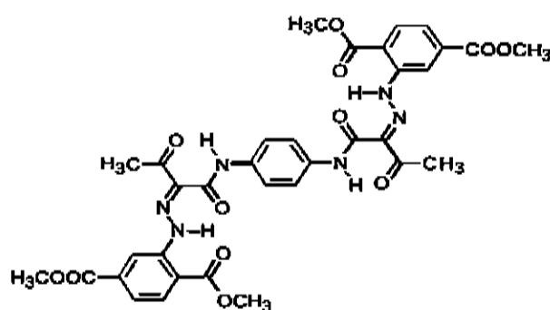
Structural Formula (3)
