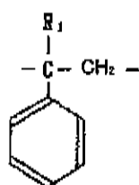
General Formula(VI)
