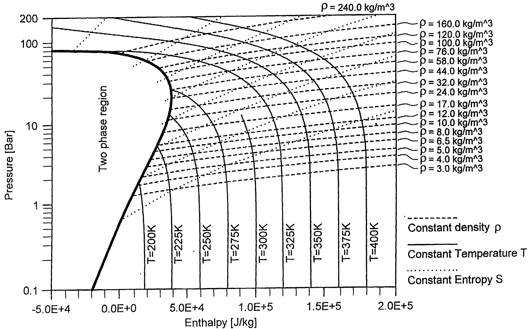
Phase Diagram for Anhydrous HCl
