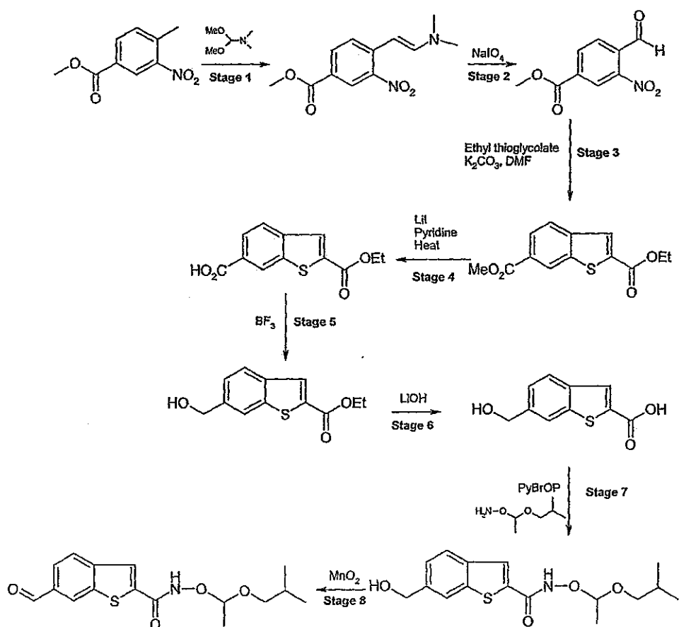
Scheme 7
