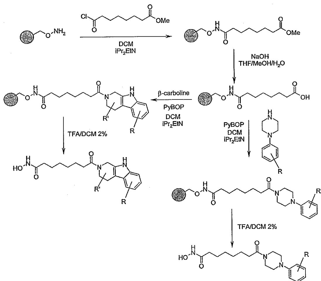
Scheme 2
