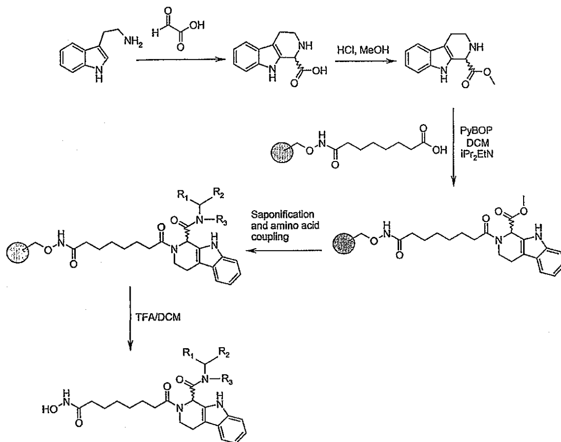
Scheme 4
