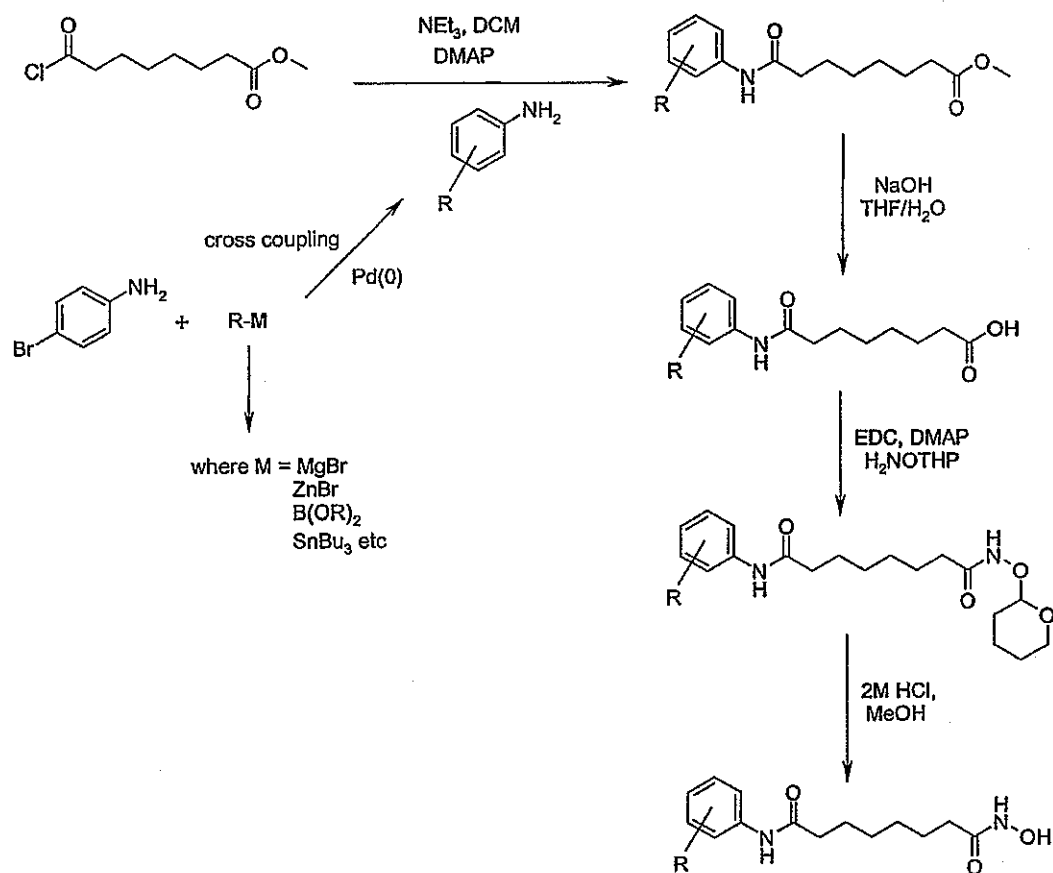
Scheme 5
