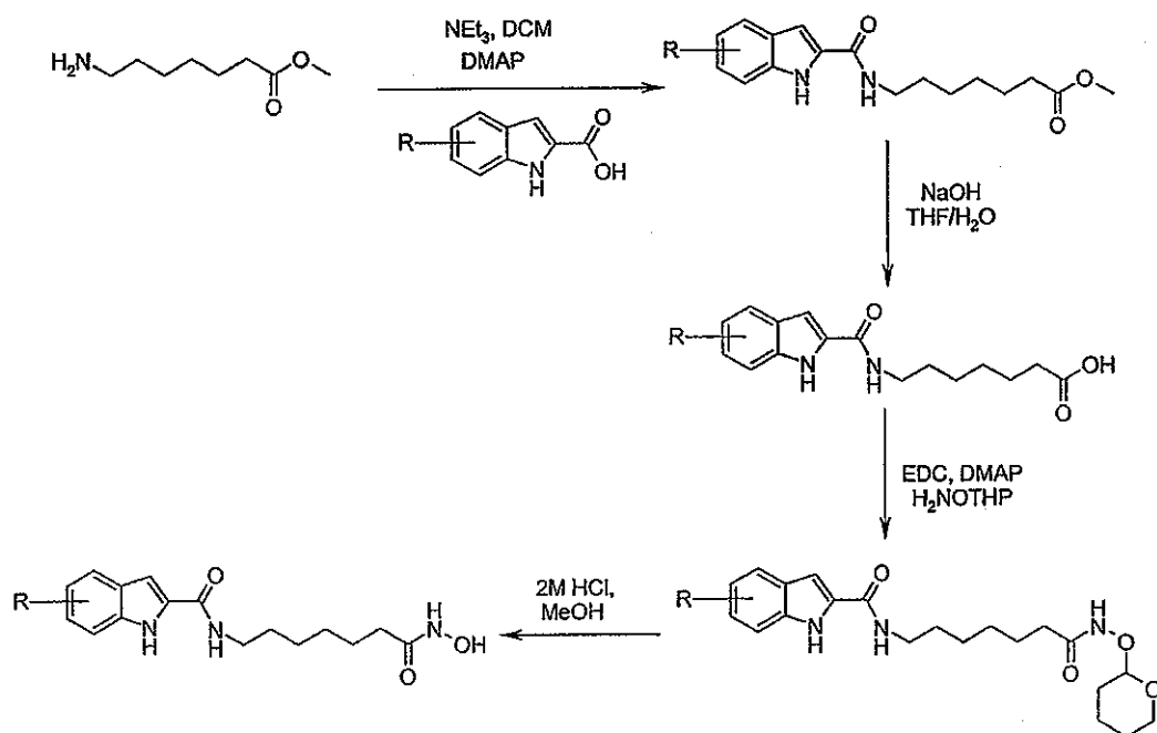
Scheme 6
