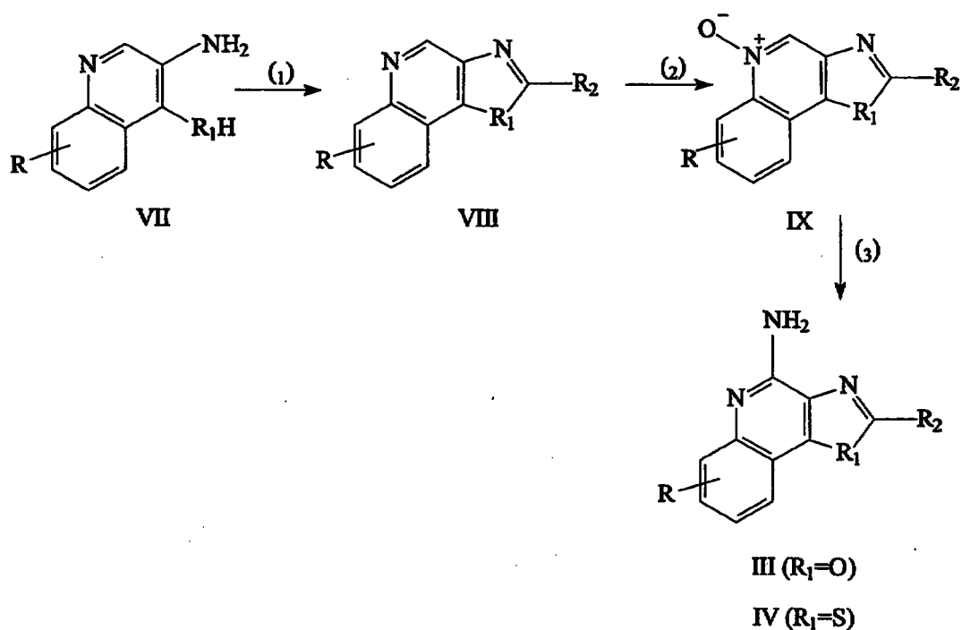
Reaction Scheme II
