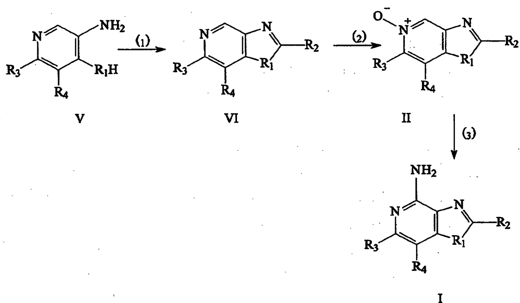
Reaction Scheme I
