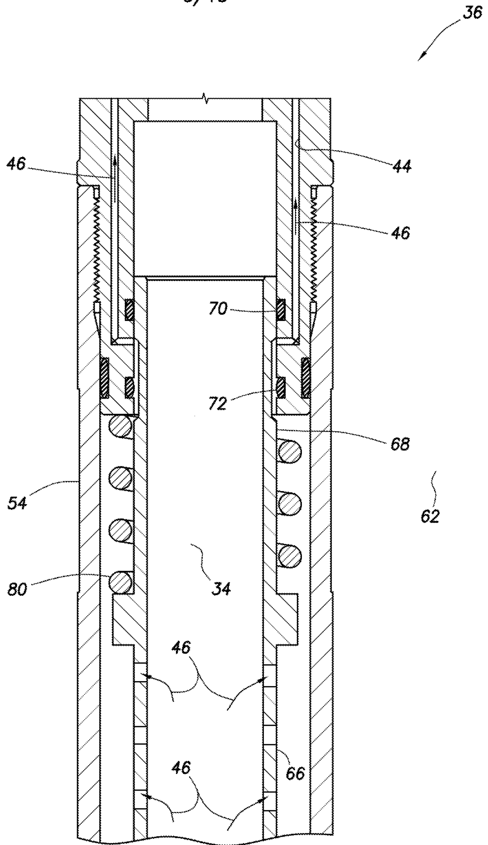
FIG. 2D
