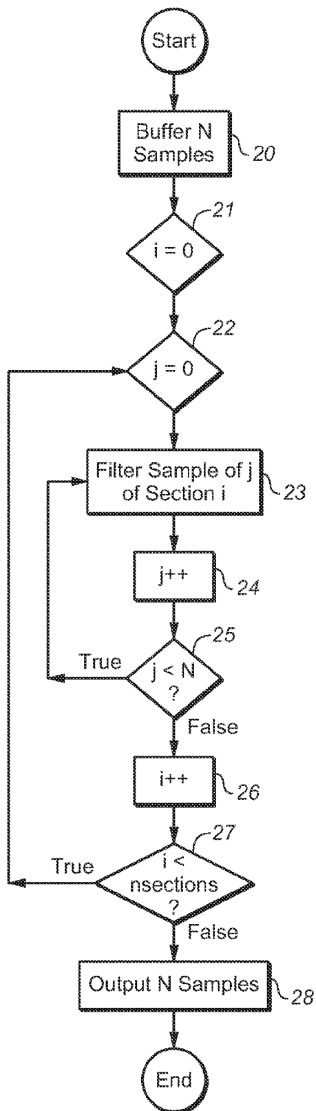
FIG. 2 (PRIOR ART)
