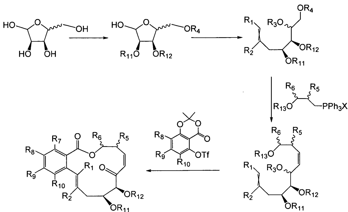
Scheme 1: Synthesis of formula (IV) from ribose – route 1
