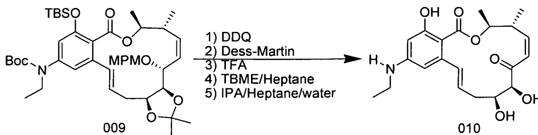
Scheme 12: Compound 010
