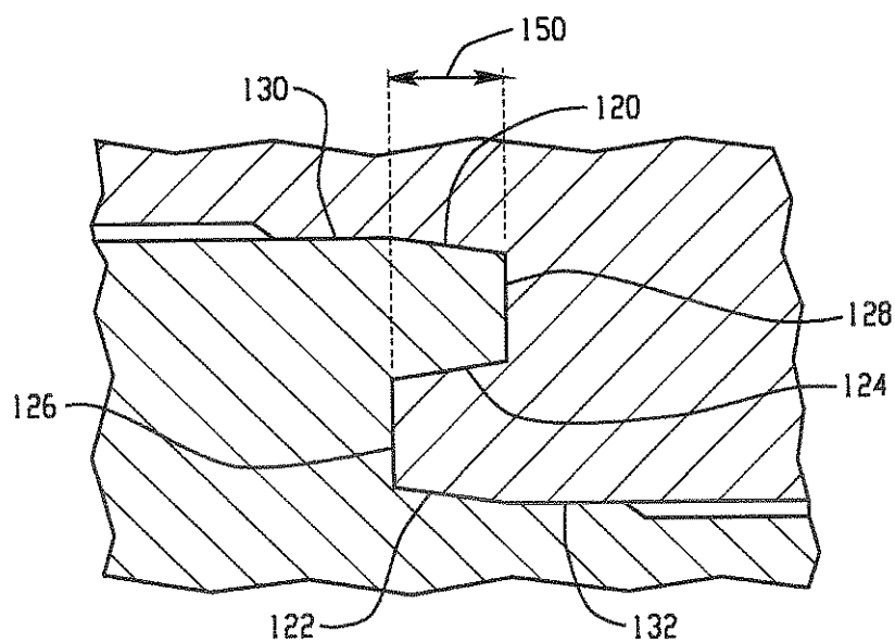
Fig. 2 PRIOR ART
