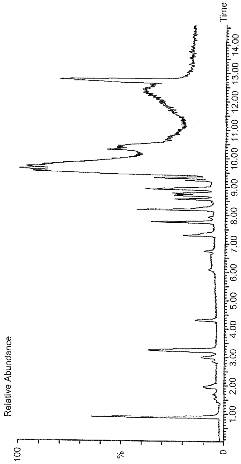
Total Ion Chromatogram of Feed Sample
