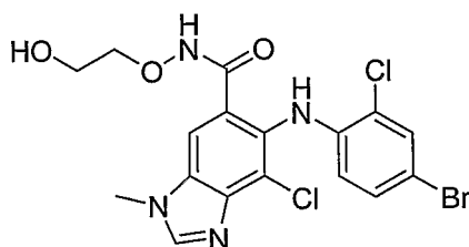
6-(4-Bromo-2-chloro-phenylamino)-7-chloro-3-methyl-3H-benzimidazole-5-carboxylic acid (2-hydroxy-ethoxy)-amide (10cc)
