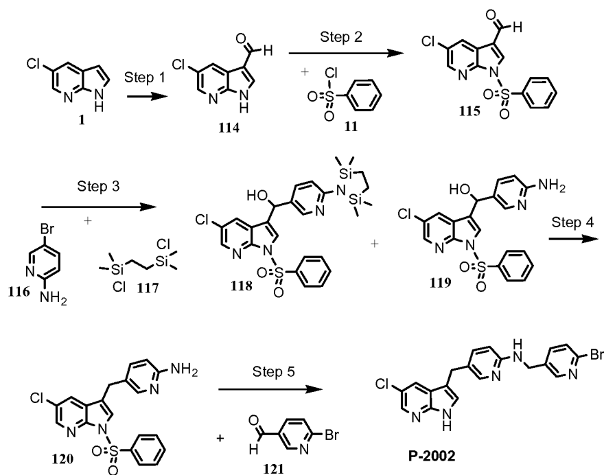
Scheme 11
