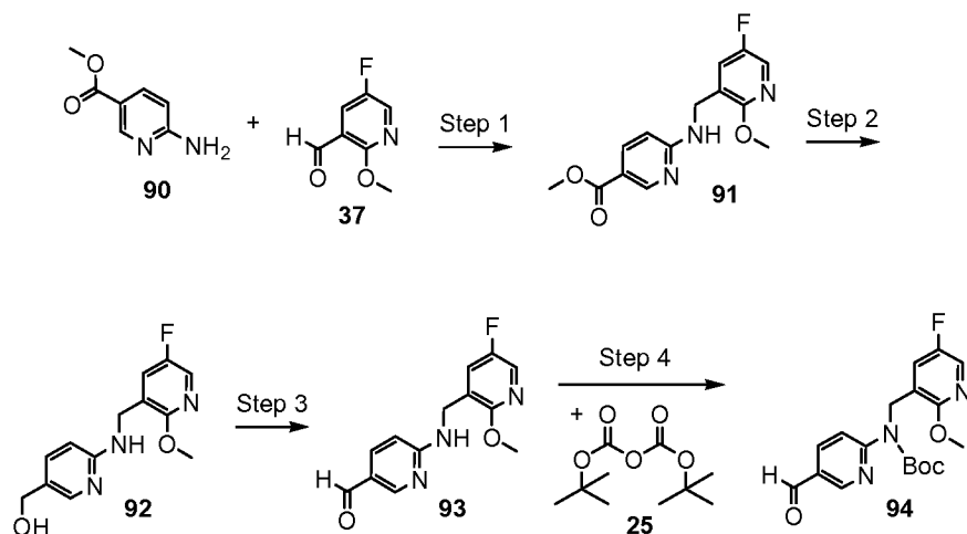
Scheme 10k
