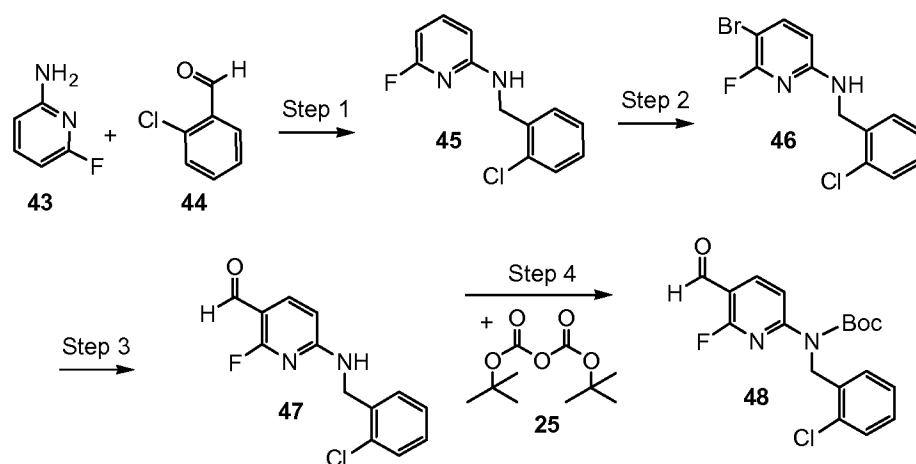
Scheme 10d
