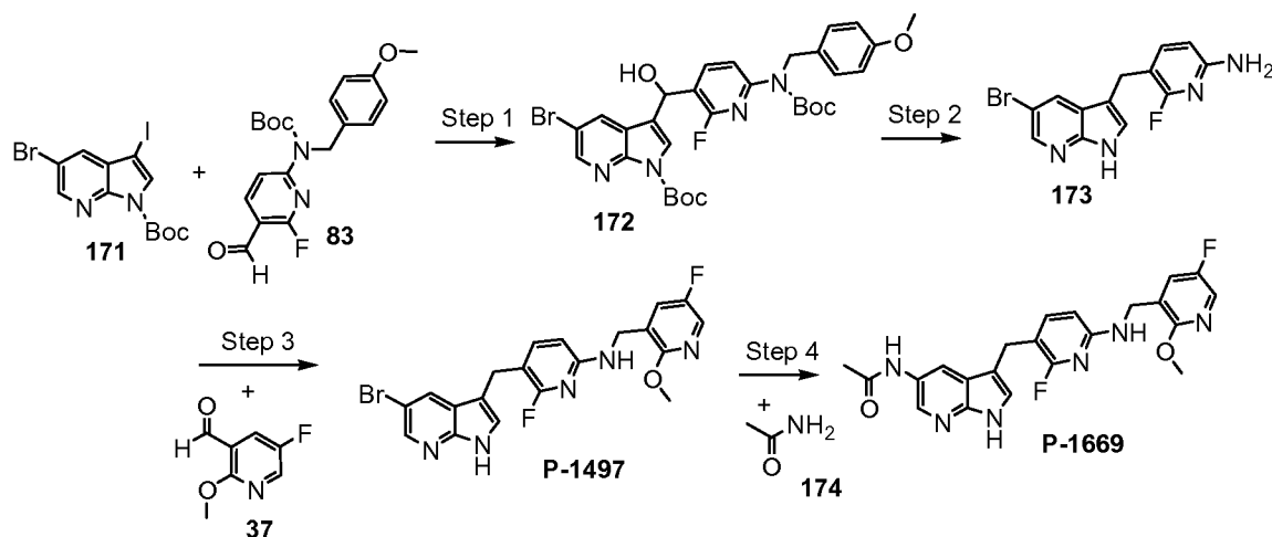
Scheme 24
