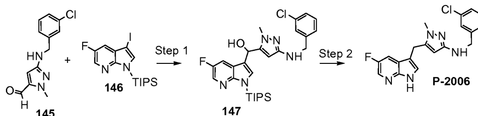
Scheme 18
