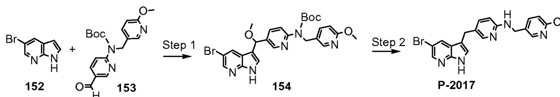
Scheme 21
