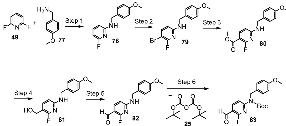
Scheme 10i
