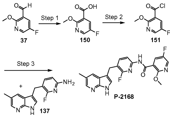
Scheme 20
