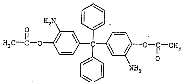
4,4'-Diacetoxy-3,3'-diaminotetraphenylmethane (bisaminophenol 5)
