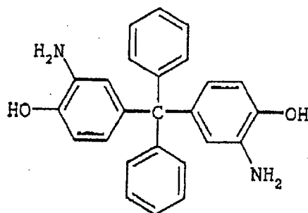
4,4'-Di-(4-amino-3-hydroxyphenoxy) tetraphenylmethane - (bisaminophenol 2)
