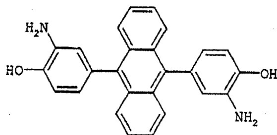
4,4'-Diamino-3,3'-dihydroxybiphenyl - (bisaminophenol 4)
