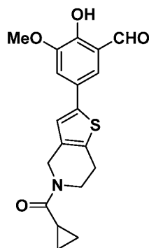
Example 14: 5-(5-(cyclopropanecarbonyl)-4,5,6,7-tetrahydrothieno[3,2-c]pyridin-2-yl)-2-hydroxy-3-methoxybenzaldehyde
