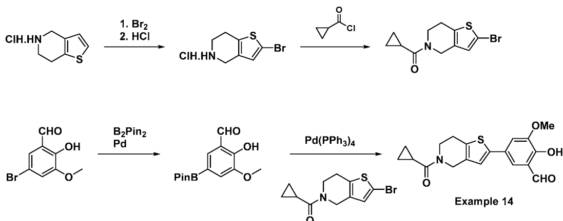
Example 14: 5-(5-(cyclopropanecarbonyl)-4,5,6,7-tetrahydrothieno[3,2-c]pyridin-2-yl)-2-hydroxy-3-methoxybenzaldehyde
