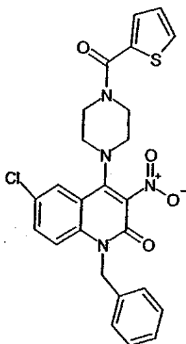
Compound 200
