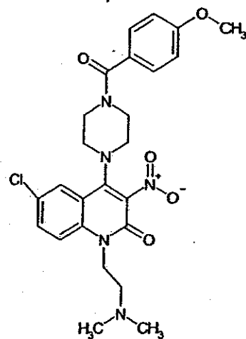
Compound 211
