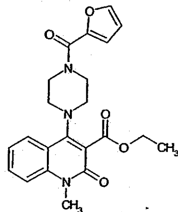
Compound 13
