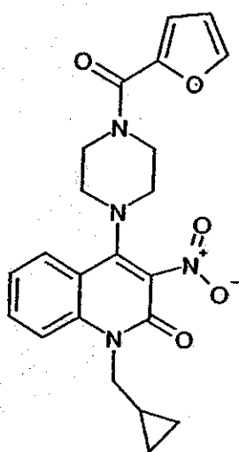
Compound 219
