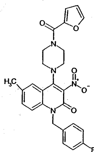
Compound 174
