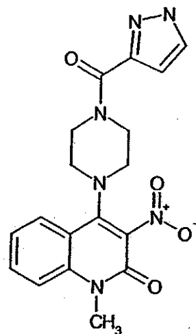
Compound 228
