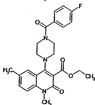
Compound 44
