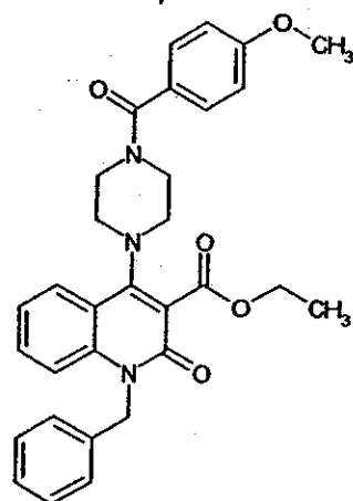
Compound 25
