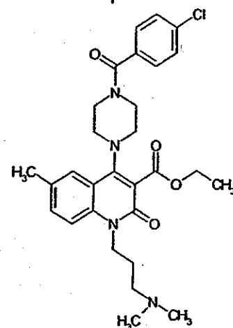
Compound 97
