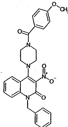
Compound 114
