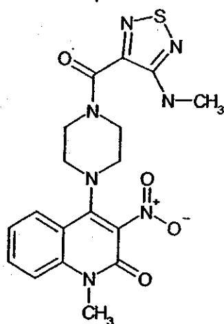
Compound 231
