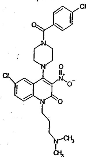
Compound 207
