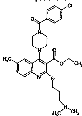
Compound 335
