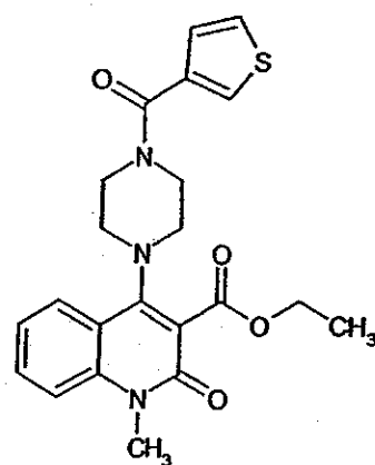
Compound 258
