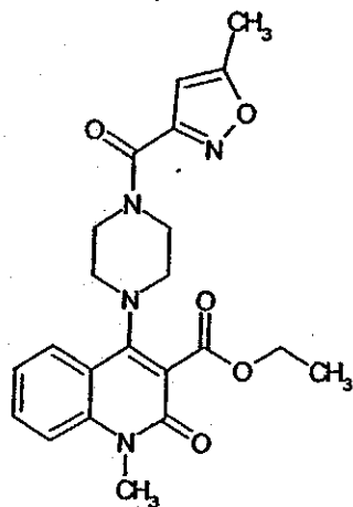
Compound 243
