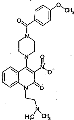
Compound 160
