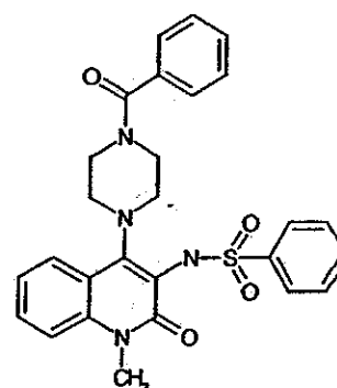
Compound 85
