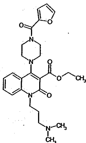
Compound 110
