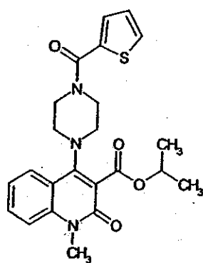
Compound 213
