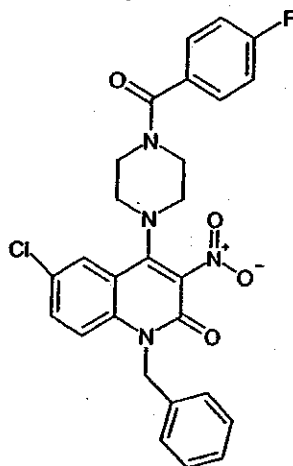
Compound 203
