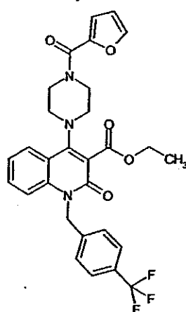
Compound 292
