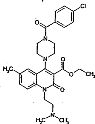
Compound 124
