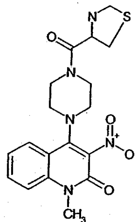
Compound 307
