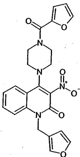
Compound 321
