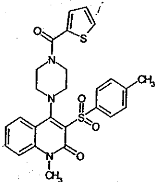
Compound 104
