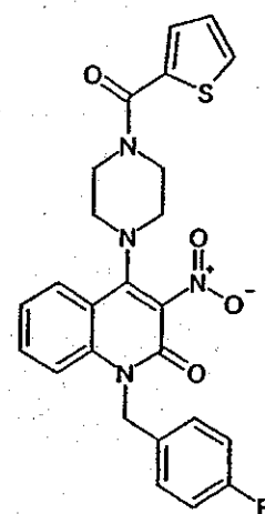
Compound 132
