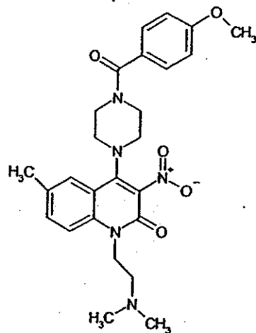
Compound 196
