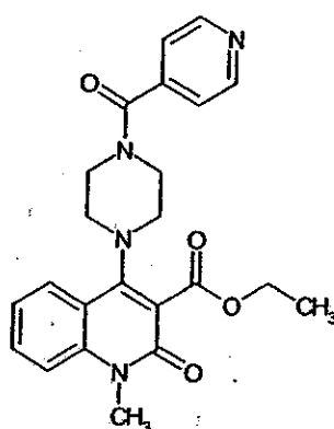
Compound 263
