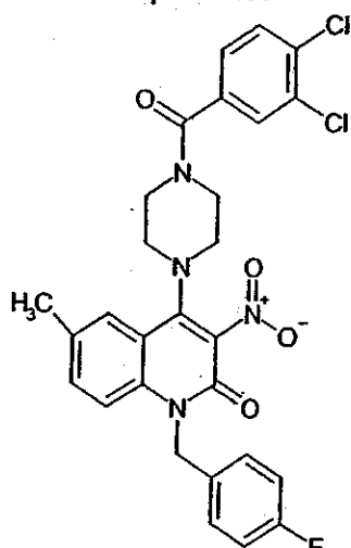
Compound 190
