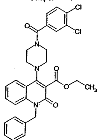
Compound 24
