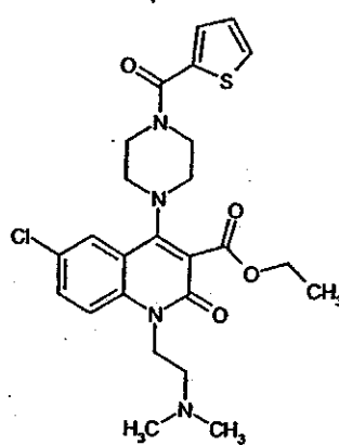
Compound 155
