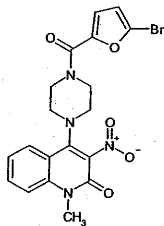
Compound 229
