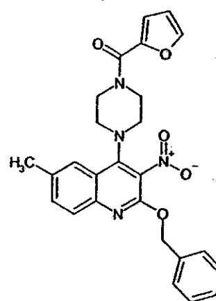
Compound 344
