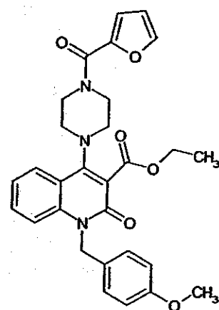
Compound 217
