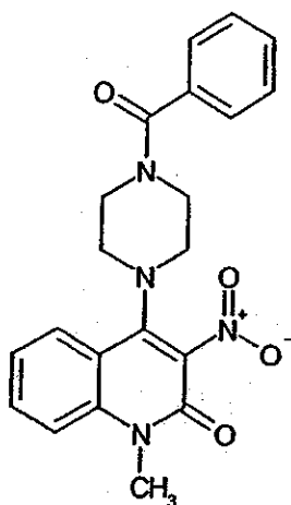
Compound 10
