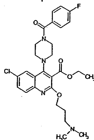
Compound 331
