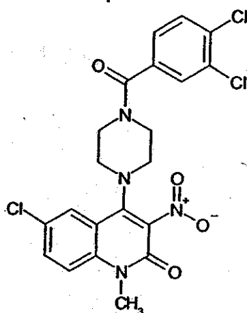
Compound 129
