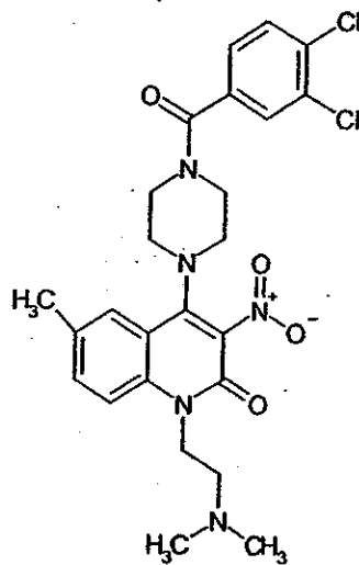
Compound 191
