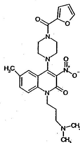
Compound 175
