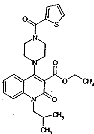
Compound 297
