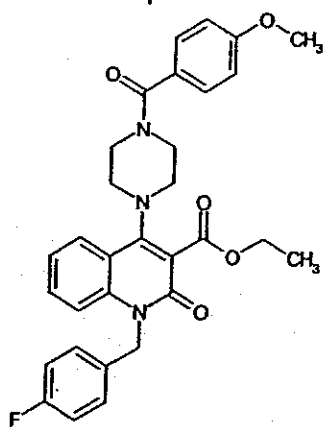
Compound 20
