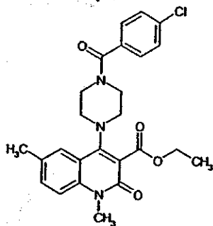
Compound 68
