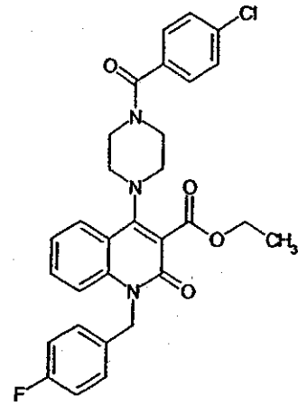
Compound 18
