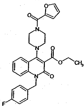
Compound 15
