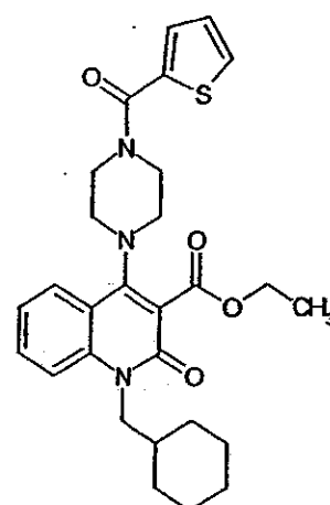
Compound 246
