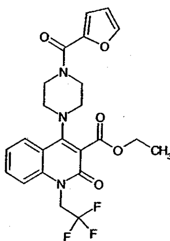
Compound 239
