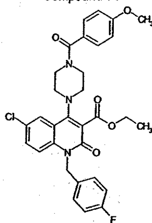
Compound 70
