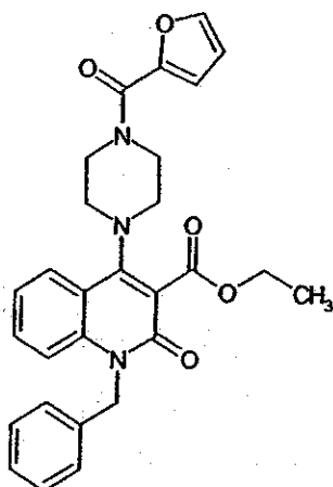
Compound 14
