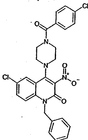
Compound 166
