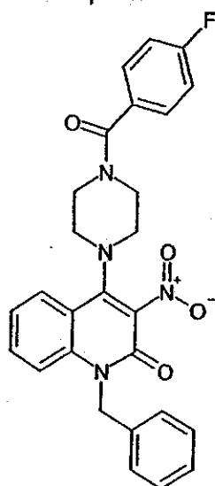
Compound 118
