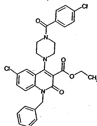
Compound 36
