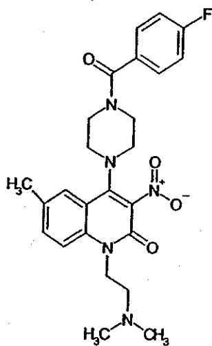
Compound 182
