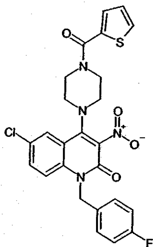
Compound 147
