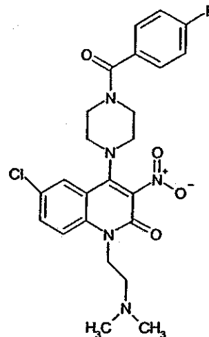
Compound 204
