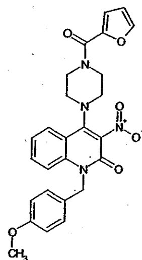
Compound 271
