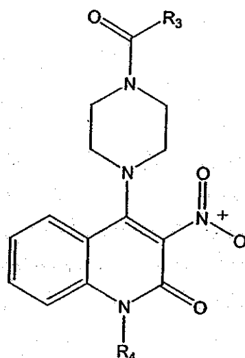
(Formula AIV)
