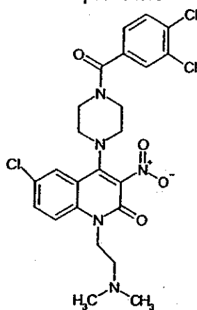
Compound 209
