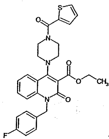
Compound 16
