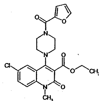
Compound 72
