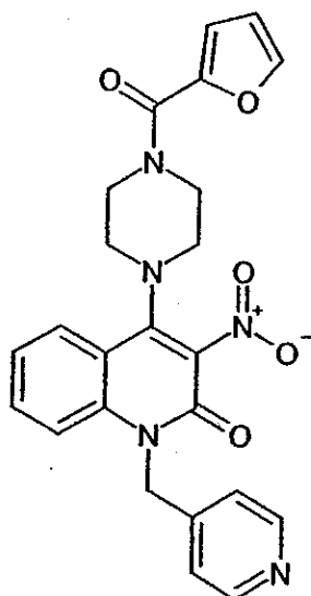
Compound 322
