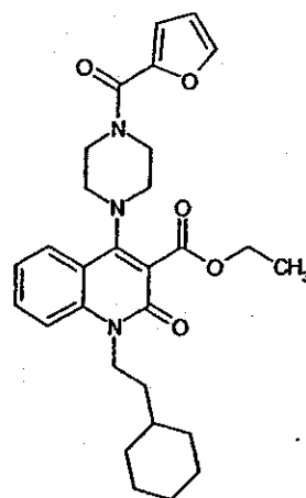
Compound 216
