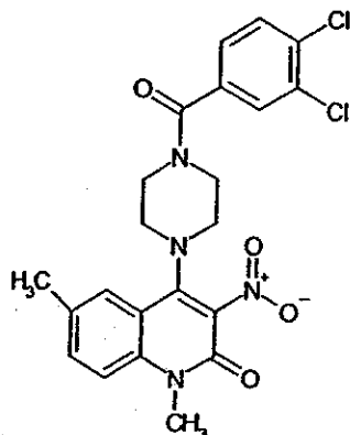
Compound 188
