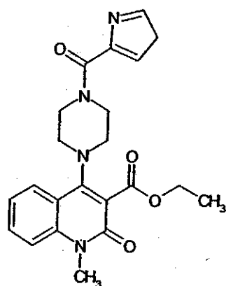
Compound 237
