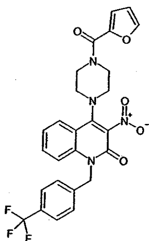
Compound 272
