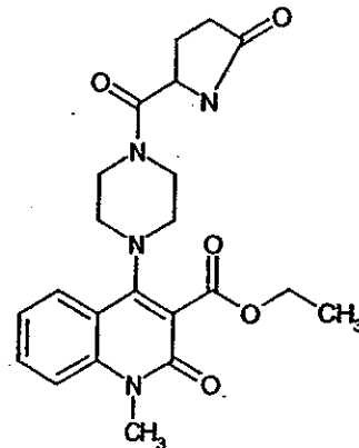
Compound 289
