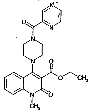
Compound 301
