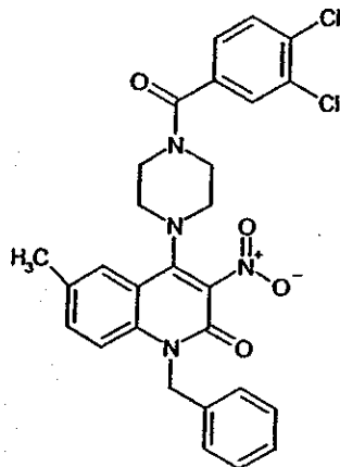
Compound 189
