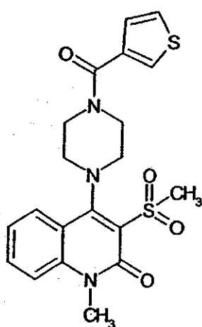
Compound 99
