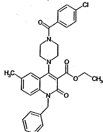
Compound 30
