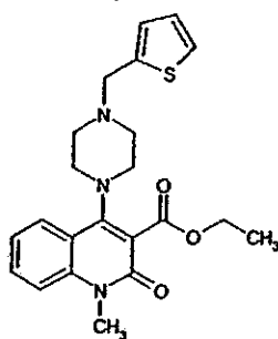
Compound 250
