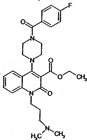
Compound 87
