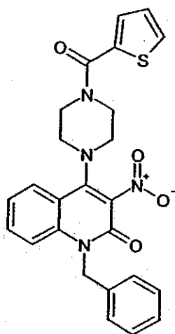
Compound 131
