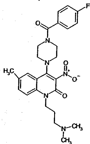
Compound 183
