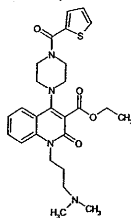
Compound 96
