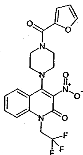
Compound 253
