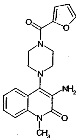
Compound 77
