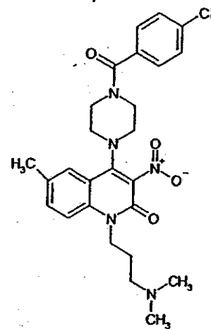
Compound 187
