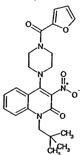
Compound 252
