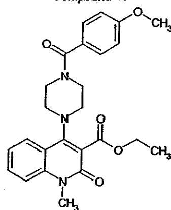
Compound 48
