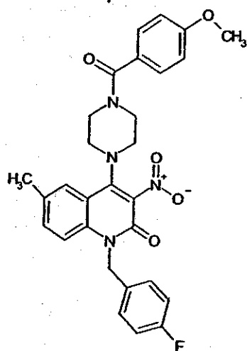
Compound 195
