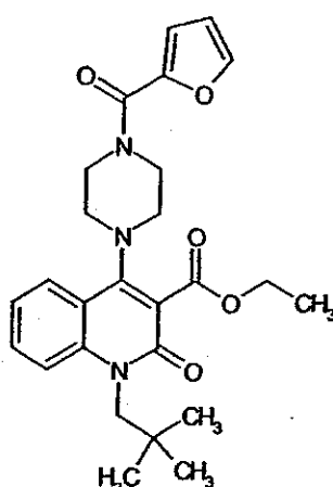
Compound 238
