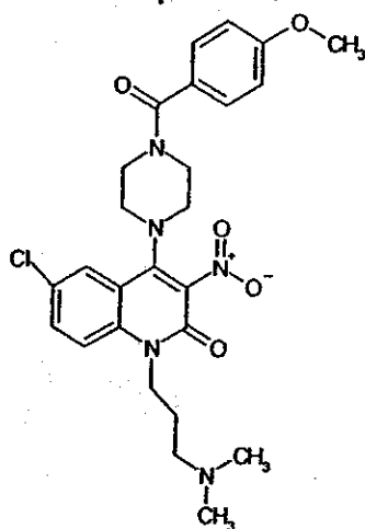
Compound 212
