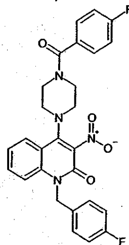
Compound 133
