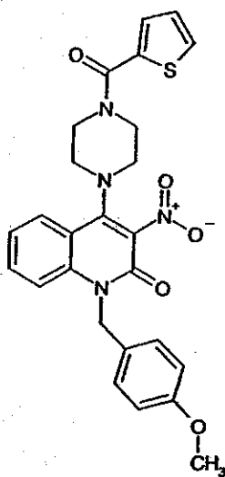
Compound 279
