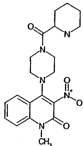
Compound 324
