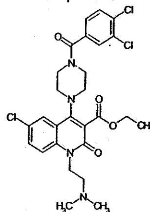
Compound 151
