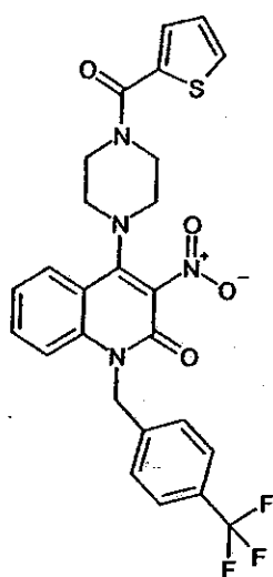
Compound 280
