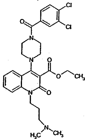
Compound 89
