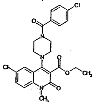
Compound 59
