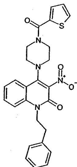
Compound 310
