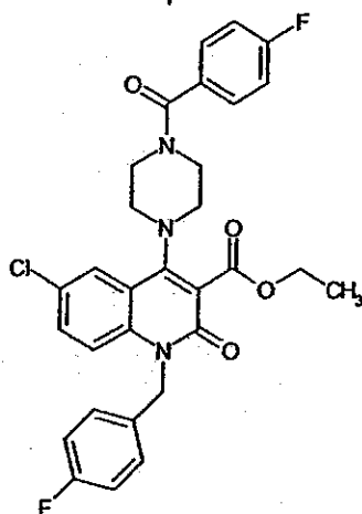
Compound 41
