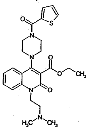
Compound 137
