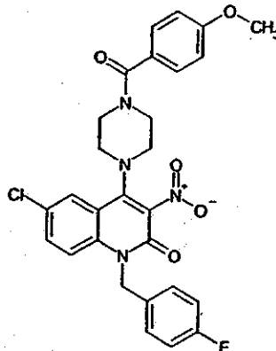
Compound 149
