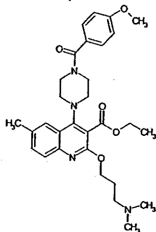
Compound 340
