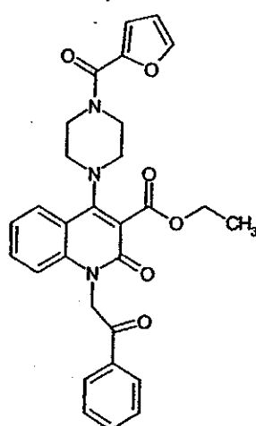
Compound 293
