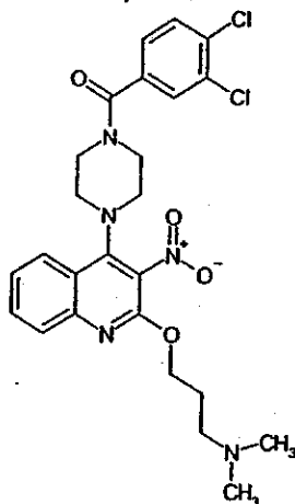
Compound 341
