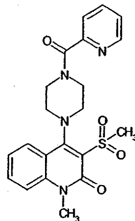
Compound 102
