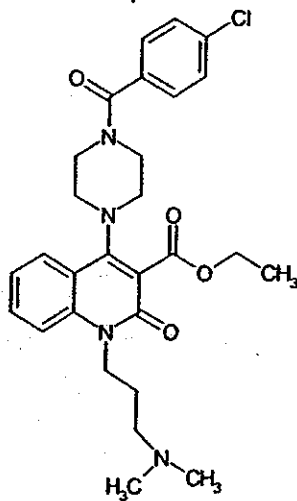
Compound 88
