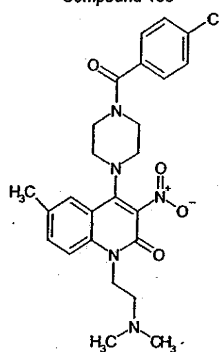
Compound 186
