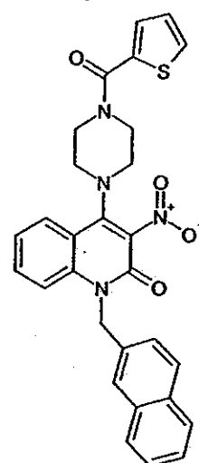
Compound 282
