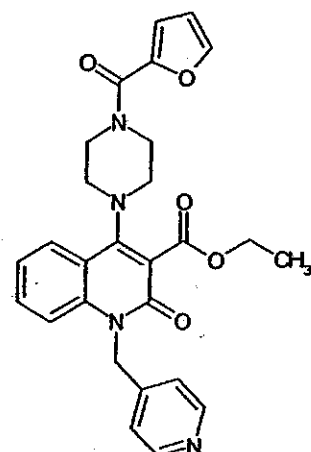
Compound 313
