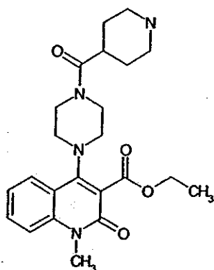
Compound 296
