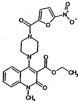
Compound 257
