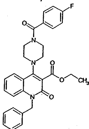
Compound 22
