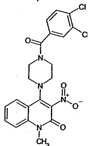
Compound 120
