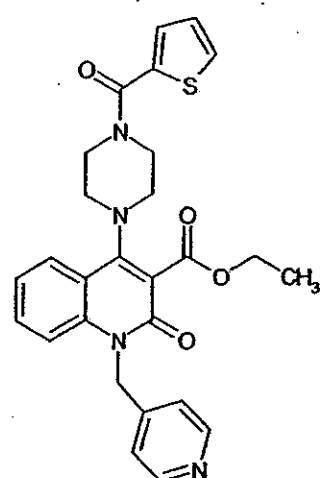
Compound 318
