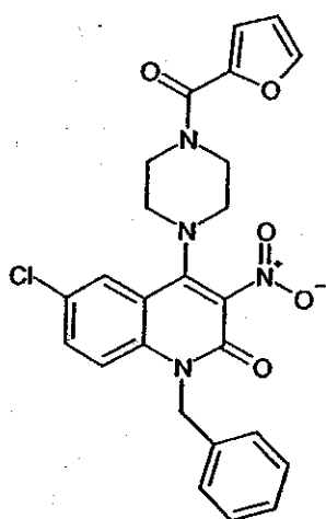
Compound 165
