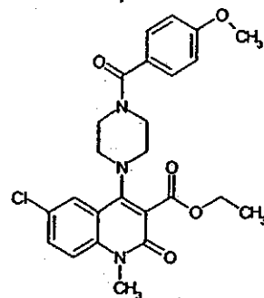
Compound 61
