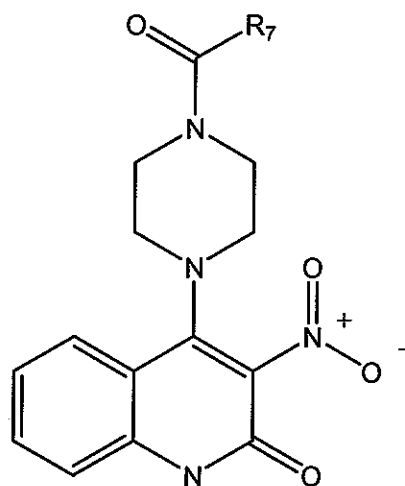
(Formula AIII)
