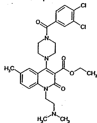
Compound 168
