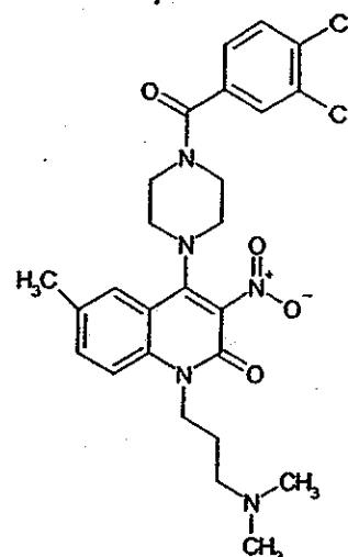
Compound 192
