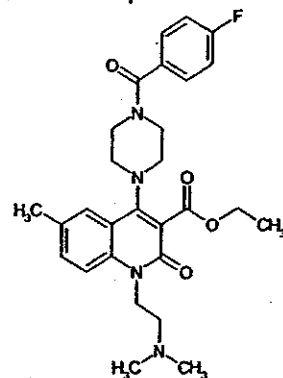
Compound 66
