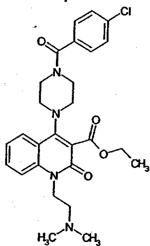
Compound 153
