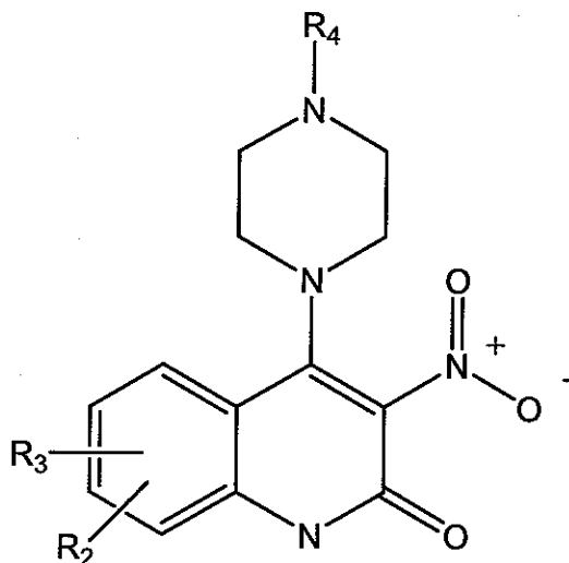
(Formula AIIIa)
