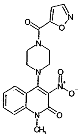
Compound 308
