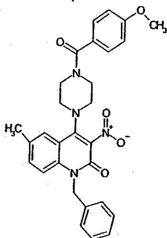
Compound 194
