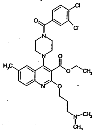
Compound 342
