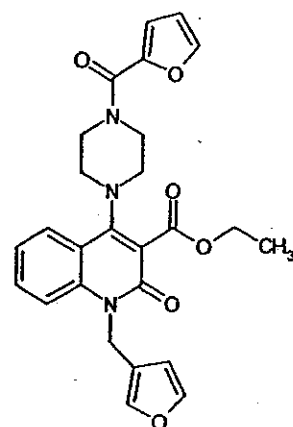
Compound 312
