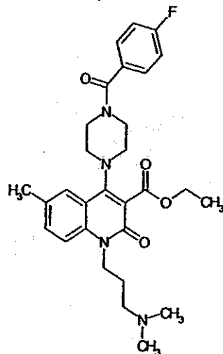
Compound 113
