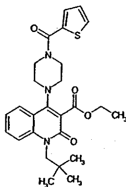
Compound 244
