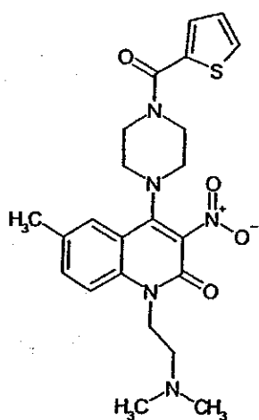
Compound 164
