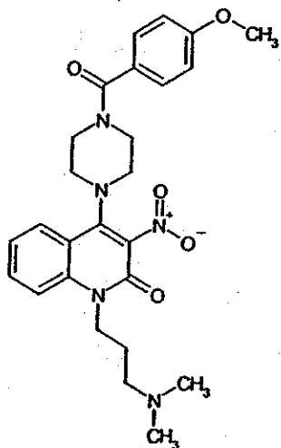
Compound 141
