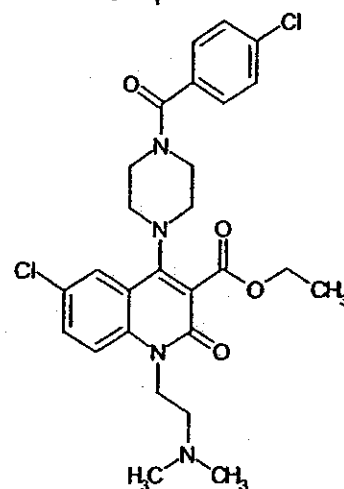
Compound 150
