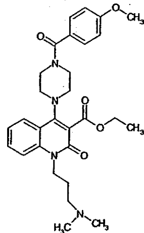
Compound 90
