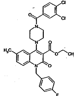
Compound 54
