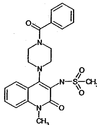
Compound 79
