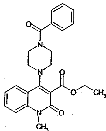
Compound 12
