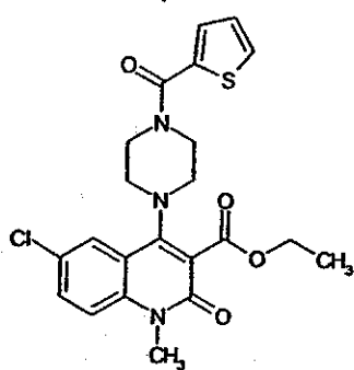
Compound 57
