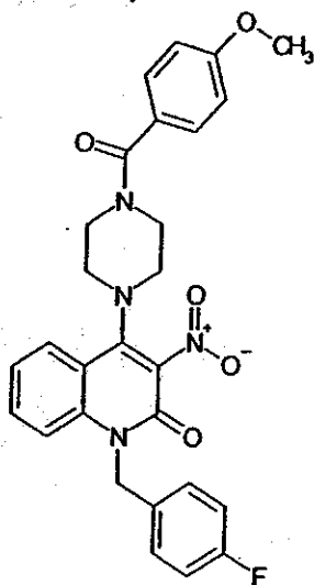
Compound 116
