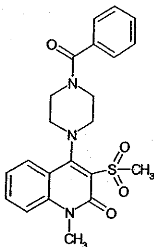
Compound 82
