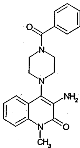
Compound 76
