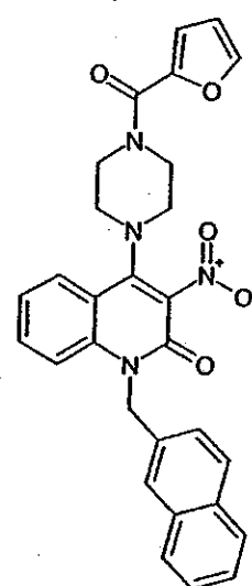
Compound 306
