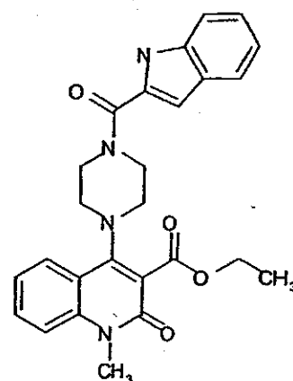
Compound 264
