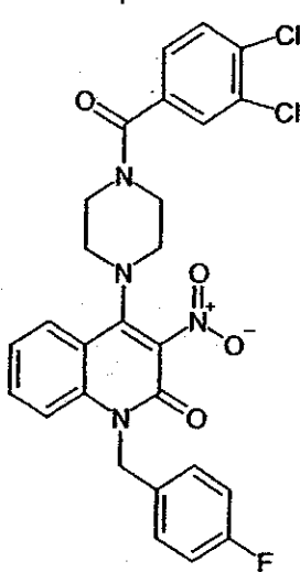
Compound 136
