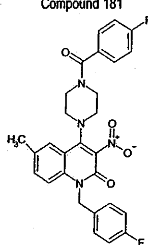
Compound 181
