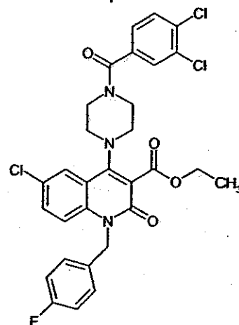
Compound 43
