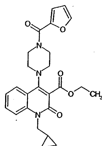
Compound 240
