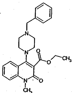
Compound 218
