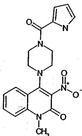
Compound 269
