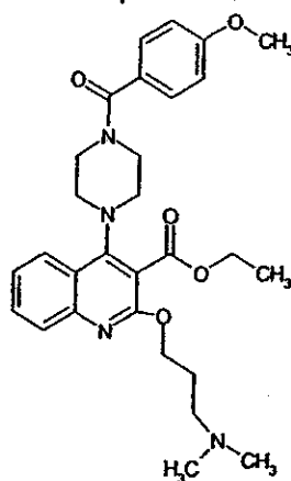
Compound 329
