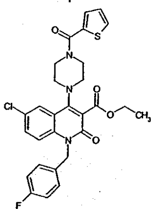
Compound 40
