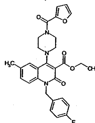
Compound 49
