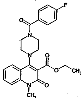
Compound 71
