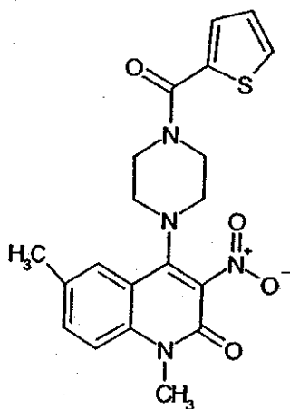
Compound 176
