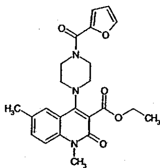
Compound 26
