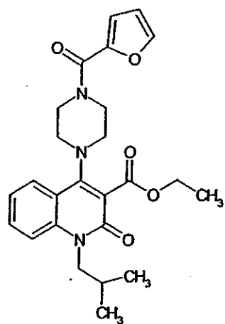
Compound 232
