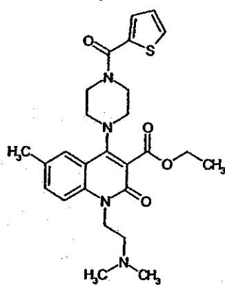
Compound 105
