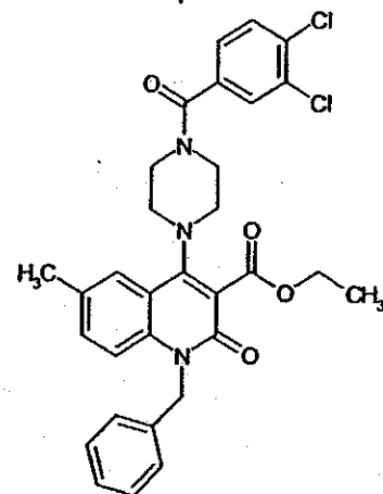
Compound 31
