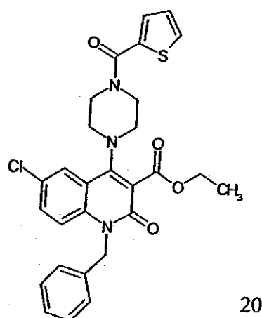
Compound 34
