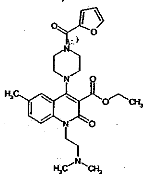
Compound 65
