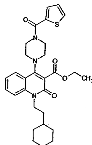
Compound 247
