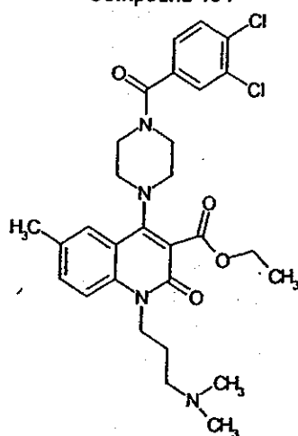
Compound 154
