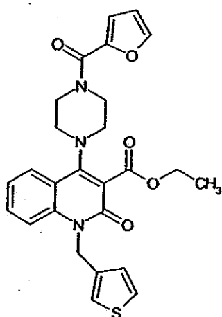
Compound 291
