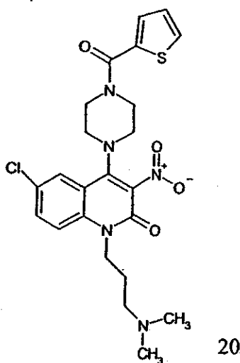
Compound 202
