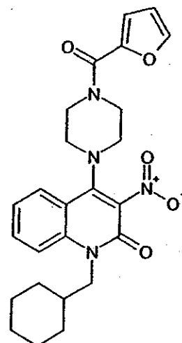
Compound 270
