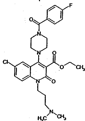
Compound 93
