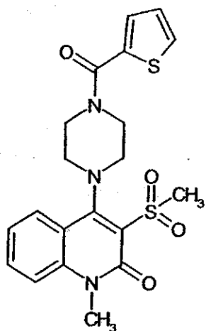
Compound 62
