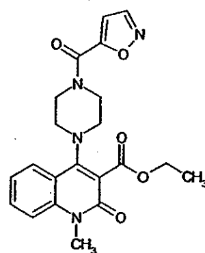
Compound 295
