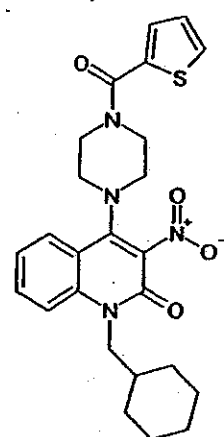
Compound 277
