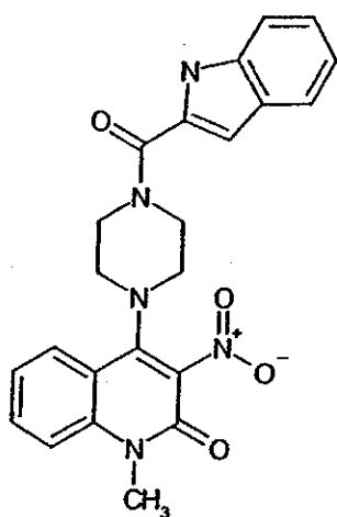
Compound 284
