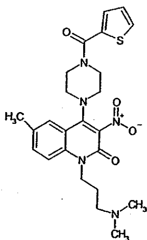
Compound 178
