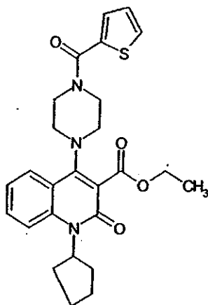
Compound 320
