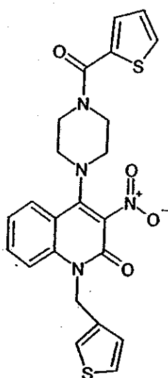
Compound 255
