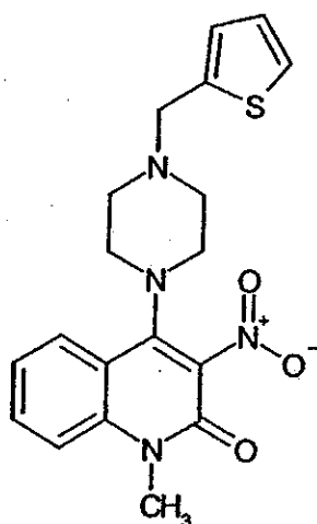
Compound 287
