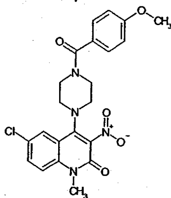
Compound 130
