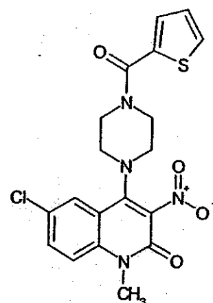
Compound 126
