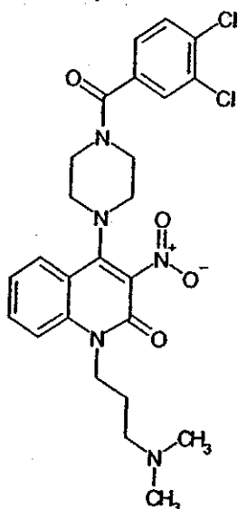
Compound 152
