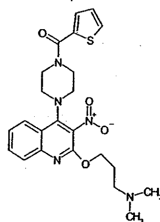
Compound 343
