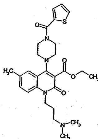
Compound 107
