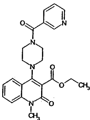
Compound 248
