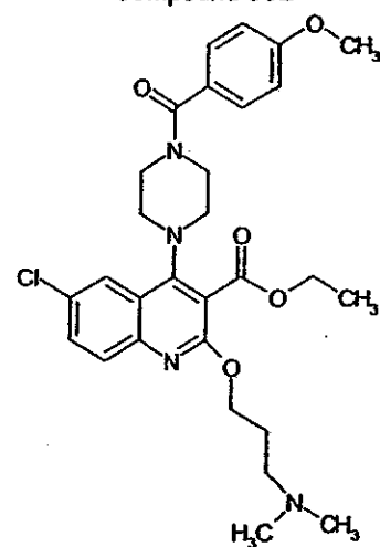
Compound 332
