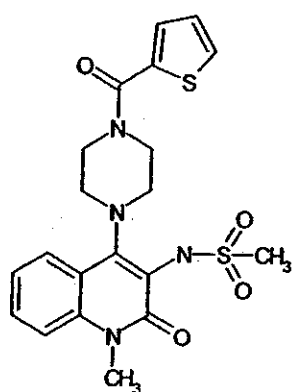
Compound 45
