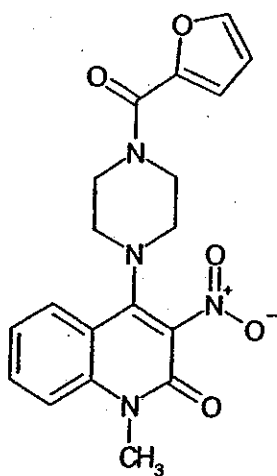
Compound 8
