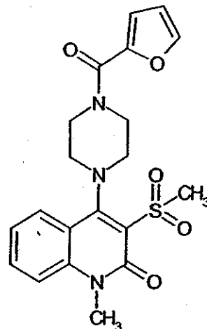
Compound 78
