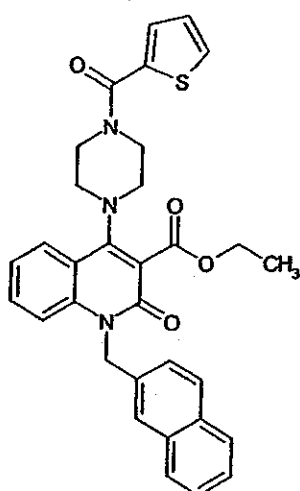
Compound 262
