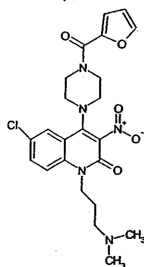
Compound 199
