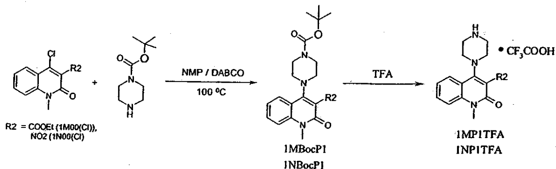
Reaction Scheme 15
