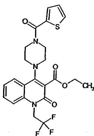
Compound 245
