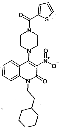
Compound 278
