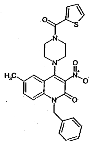
Compound 163
