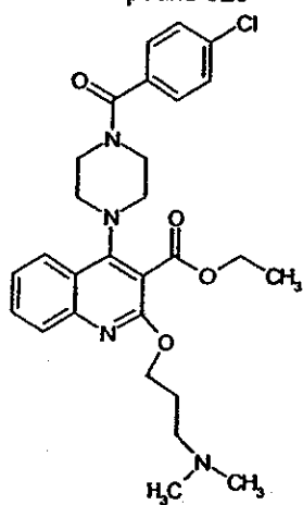
Compound 328
