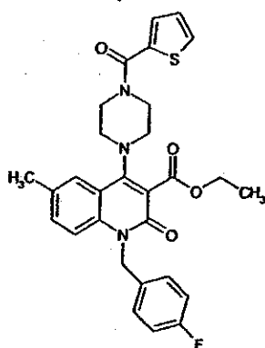
Compound 51
