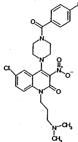
Compound 205
