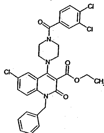
Compound 37
