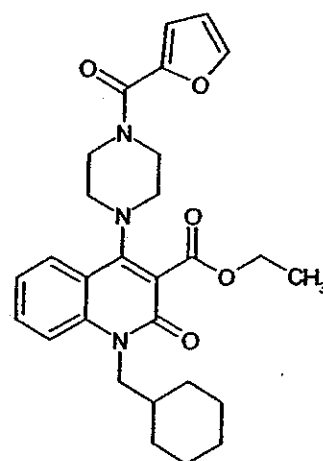
Compound 241
