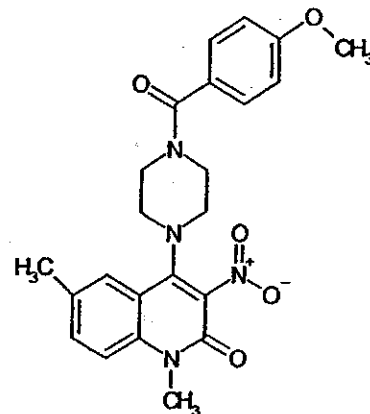
Compound 193
