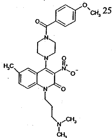
Compound 197
