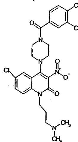
Compound 210
