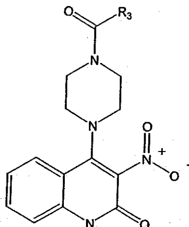
(Formula AIII)
