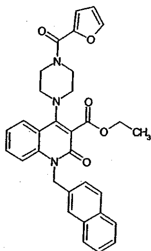
Compound 256
