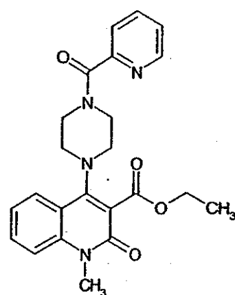
Compound 300
