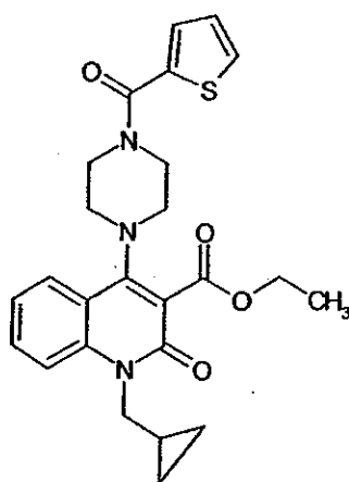
Compound 298
