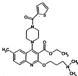
Compound 339
