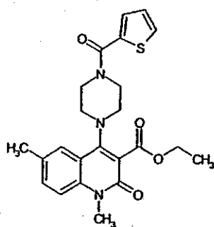
Compound 50
