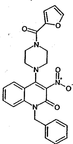
Compound 119
