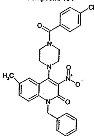
Compound 184
