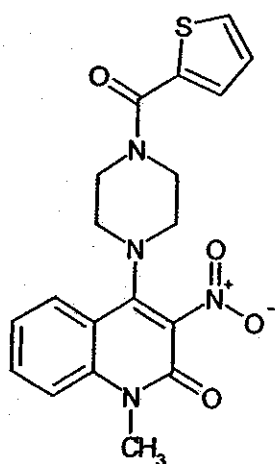
Compound 9
