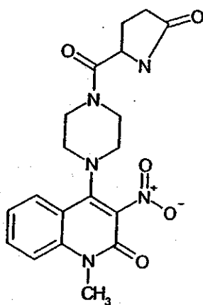
Compound 303
