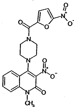
Compound 227
