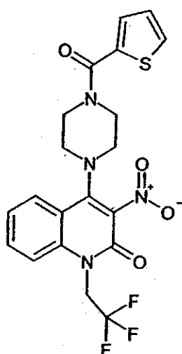
Compound 309
