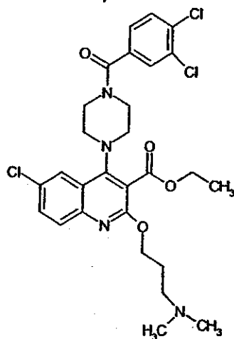
Compound 334
