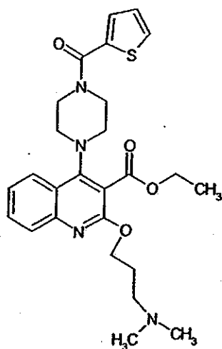
Compound 333
