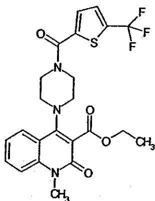
Compound 242
