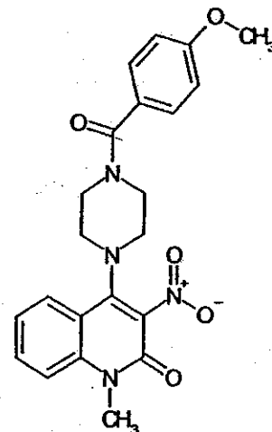
Compound 115
