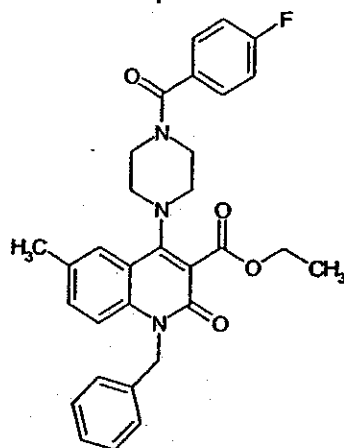
Compound 29
