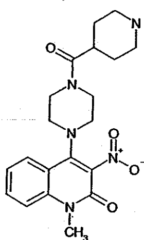
Compound 275
