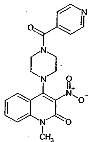
Compound 235
