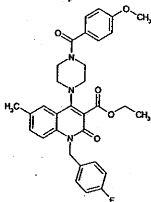
Compound 56
