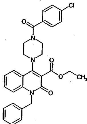
Compound 23
