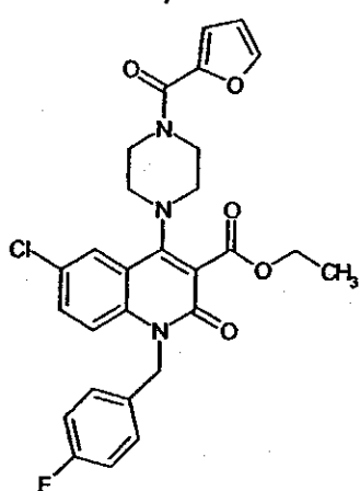
Compound 39
