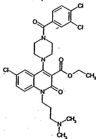
Compound 106
