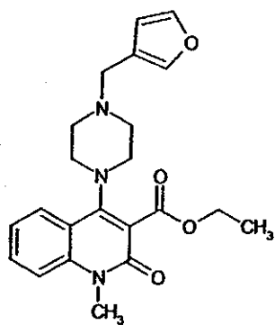
Compound 251
