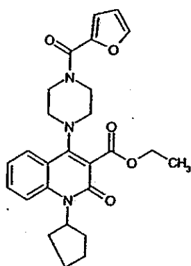
Compound 314
