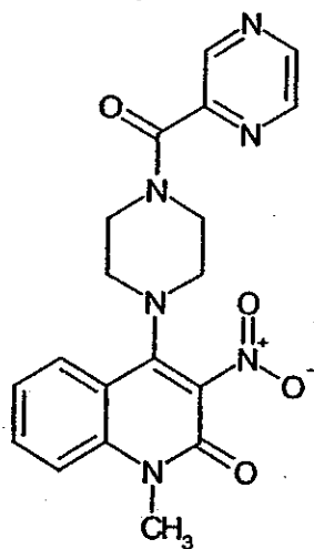
Compound 311
