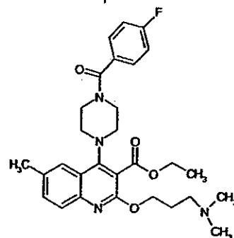
Compound 338
