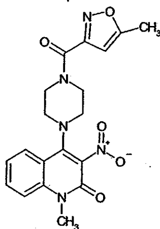
Compound 233
