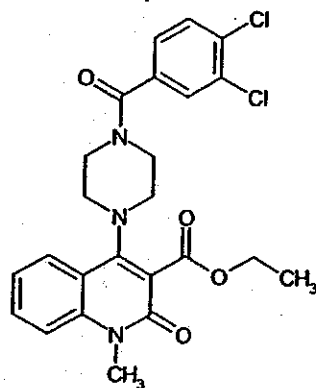
Compound 47
