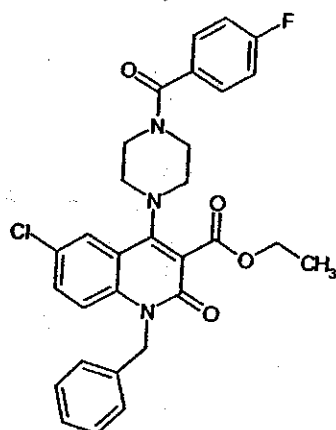
Compound 35
