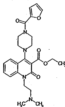
Compound 108
