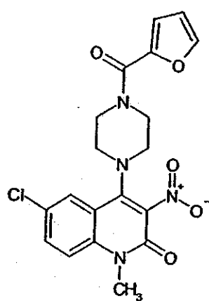
Compound 125
