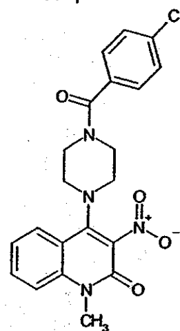
Compound 121
