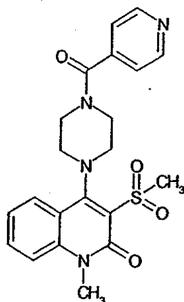
Compound 100
