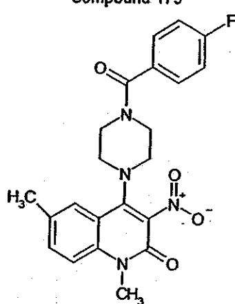
Compound 179
