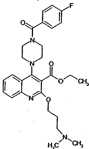
Compound 327
