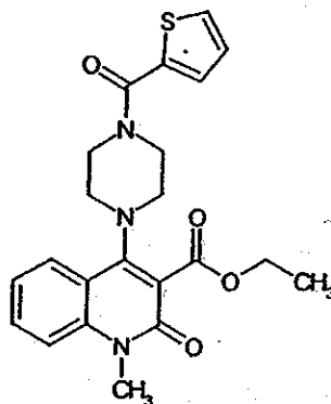
Compound 11
