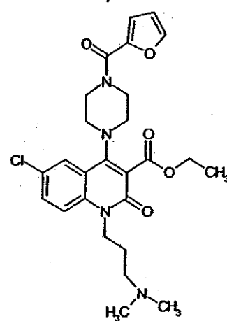
Compound 91
