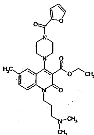
Compound 112
