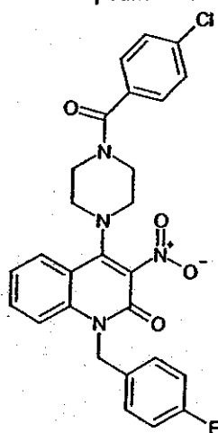
Compound 122
