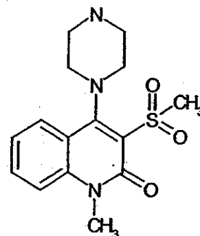
Compound 103
