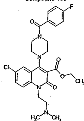
Compound 156
