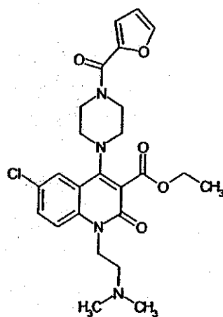
Compound 111
