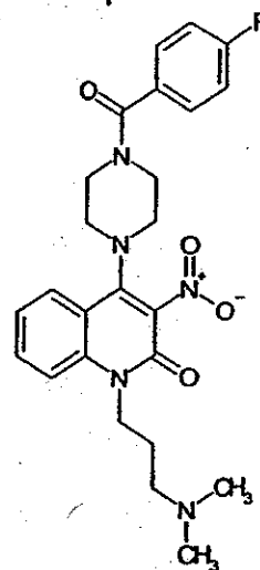
Compound 139
