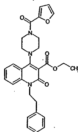
Compound 294
