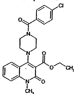
Compound 46
