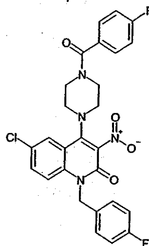
Compound 144
