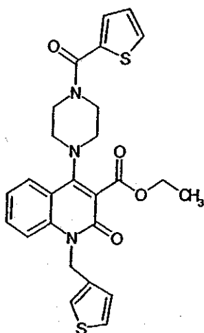
Compound 224
