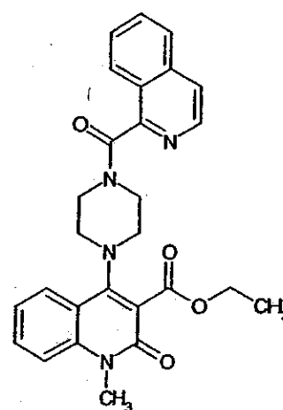
Compound 265
