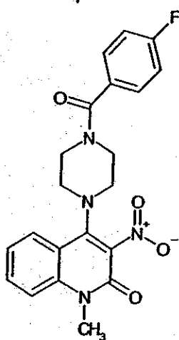
Compound 123
