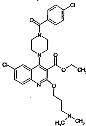
Compound 336
