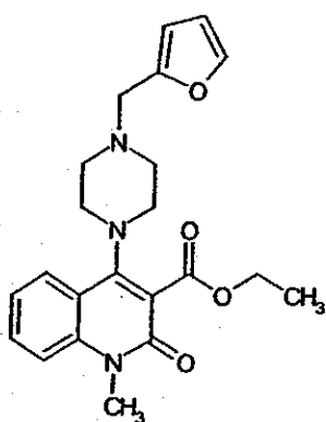
Compound 249
