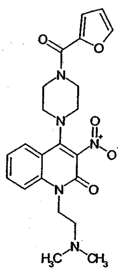
Compound 169
