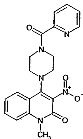
Compound 234
