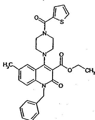
Compound 28
