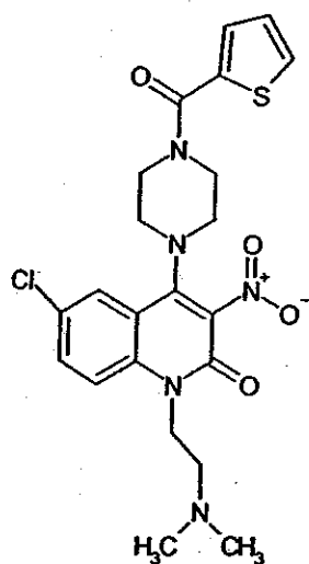
Compound 201
