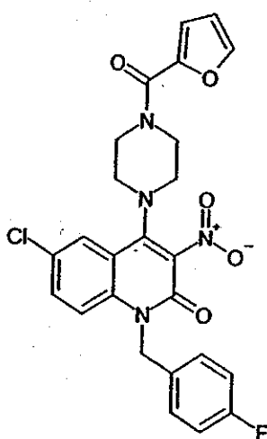
Compound 143
