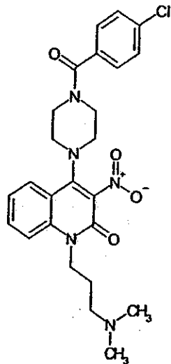
Compound 140
