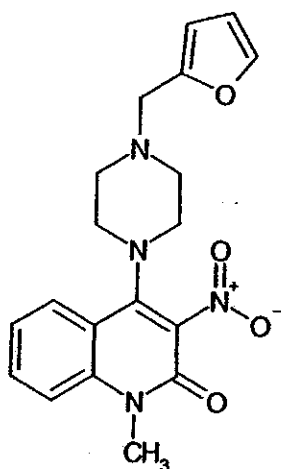
Compound 286
