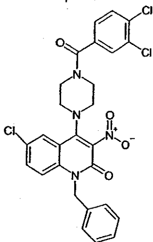
Compound 208
