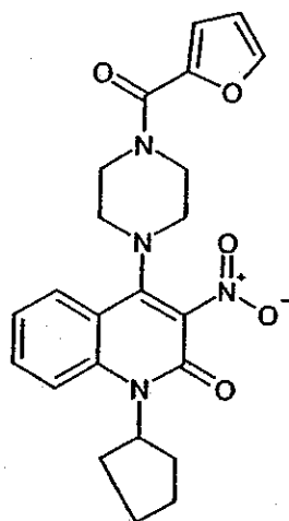
Compound 323
