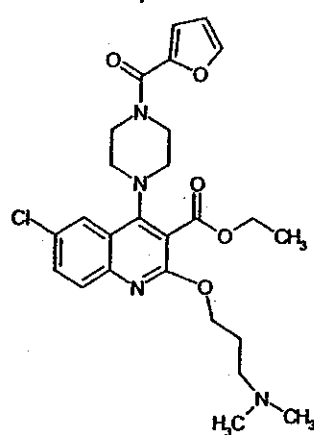
Compound 330
