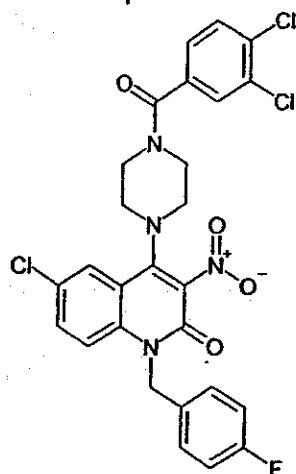
Compound 148
