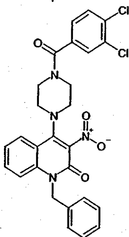
Compound 135
