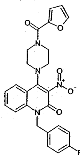
Compound 138
