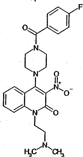
Compound 171
