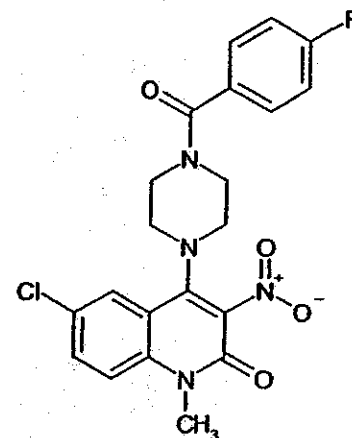
Compound 127
