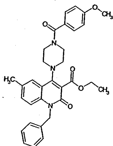
Compound 32 10
