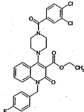
Compound 19
