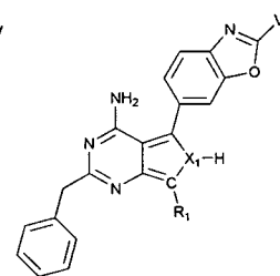
Subclass 15b
