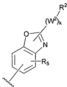
Formula A-1
