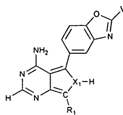
Subclass 1b
