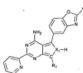
Subclass 8b
