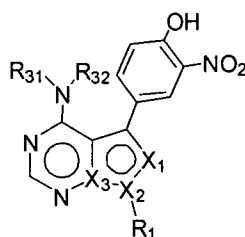
Formula 3-2
