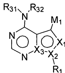
Formula C
