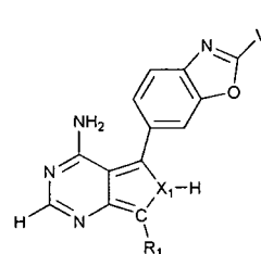
Subclass 9b
