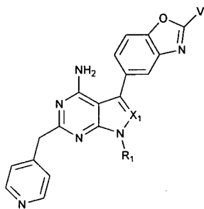
Subclass 7a
