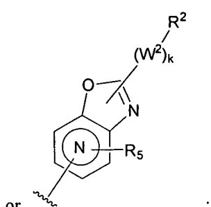
Formula A-2
