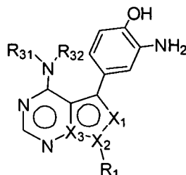
Formula 3-3
