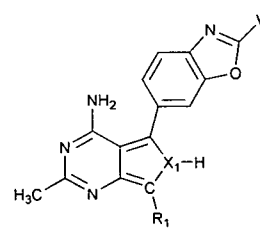
Subclass 10b
