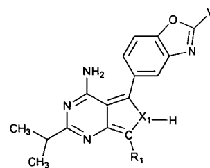
Subclass 3b
