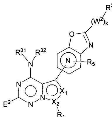
Formula II-B-2
