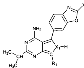
Subclass 11b
