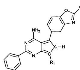
Subclass 5b
