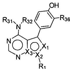
Formula 3-3'
