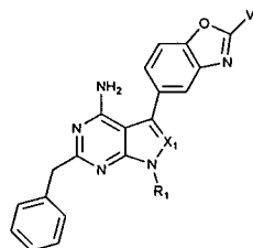
Subclass 6a
