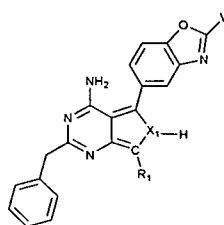
Subclass 6b
