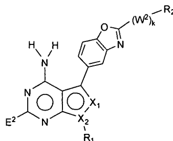
Formula II-A-1a
