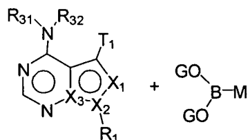
Formula A
