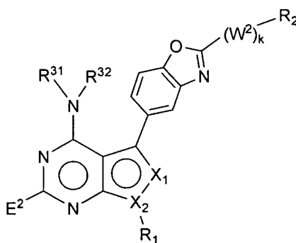
Formula II-A-1
