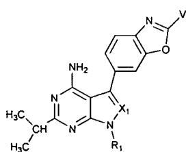
Subclass 11a
