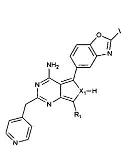
Subclass 7b
