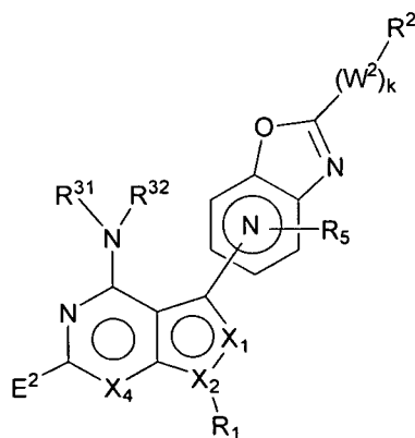
Formula IV-B-1
