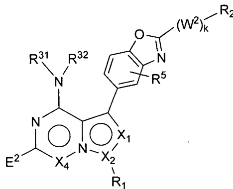
Formula IV-A-2
