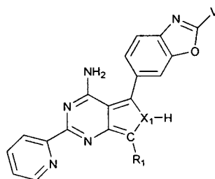
Subclass 14b
