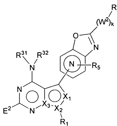
Formula II-B
