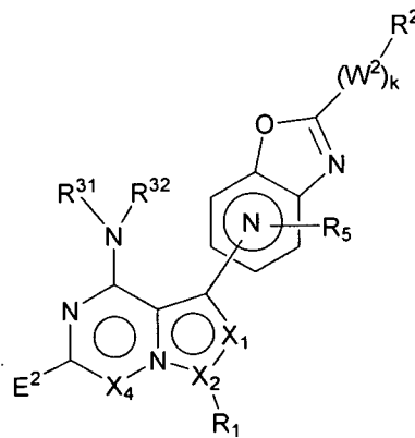
Formula IV-B-2
