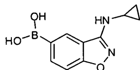
K-6-B
