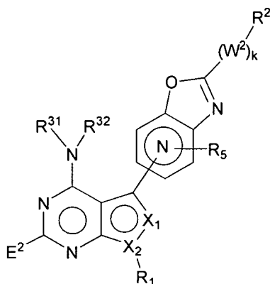
Formula II-B-1
