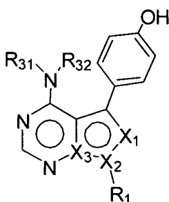
Formula 3-1
