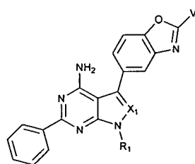
Subclass 5a
