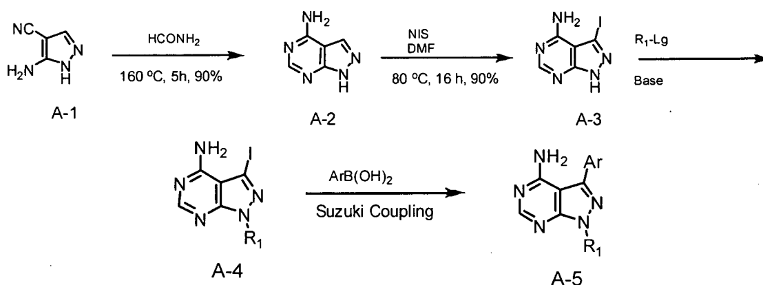
Scheme A
