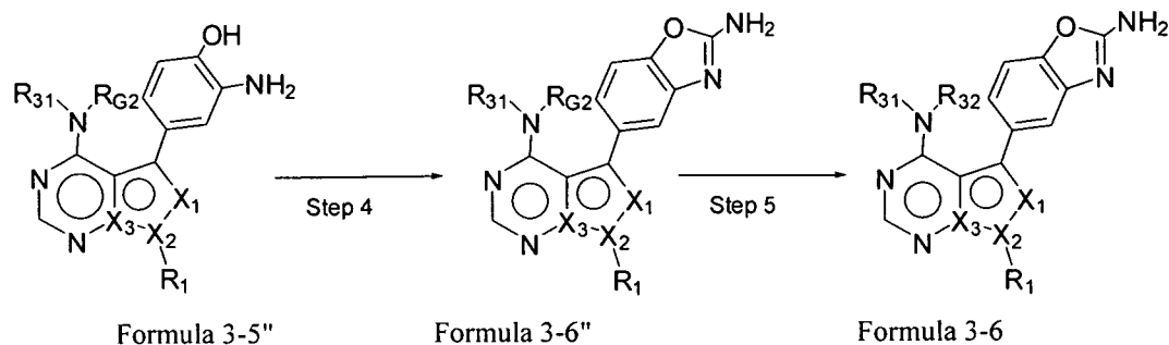
Scheme E'
