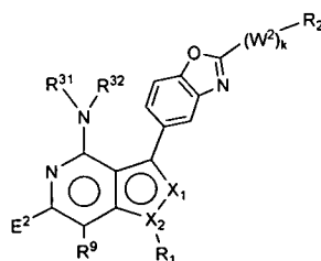
Formula IV-A-1
