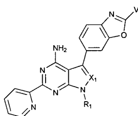
Subclass 14a
