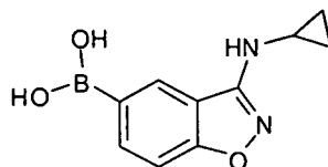
F-7-B
