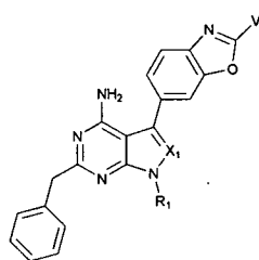
Subclass 15a
