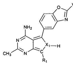
Subclass 2b
