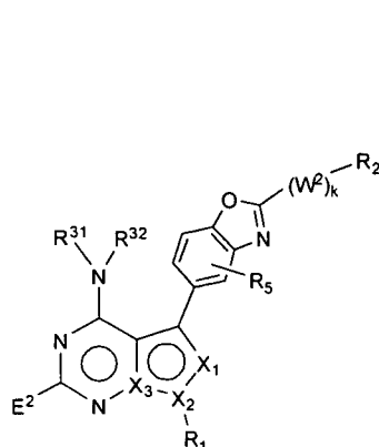
Formula II-A
