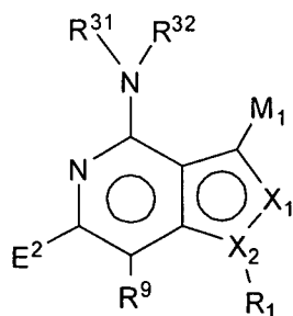
Formula III-A
