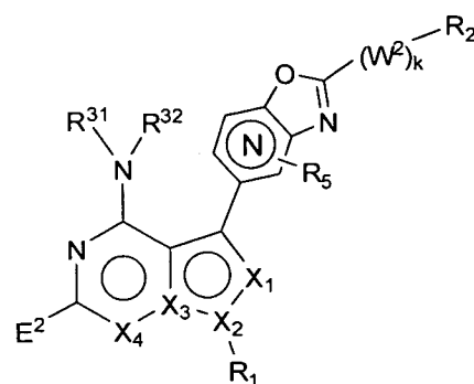
Formula IV-B
