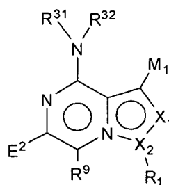
Formula III-B
