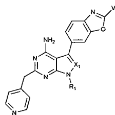
Subclass 16a
