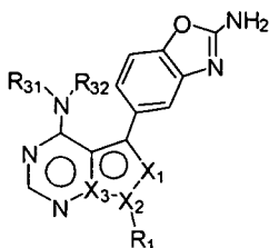
Formula 3-4
