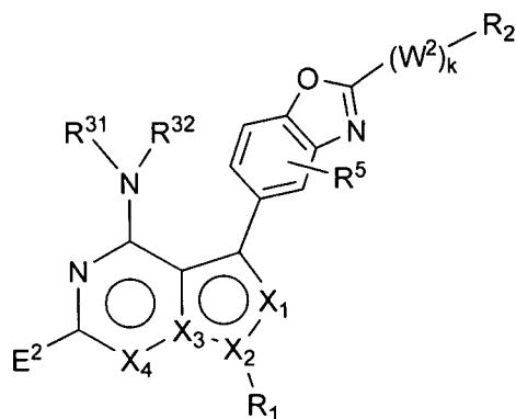
Formula IV-A
