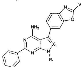
Subclass 13a
