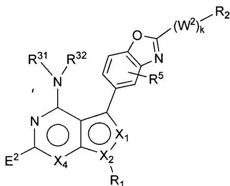
Formula IV-A-1
