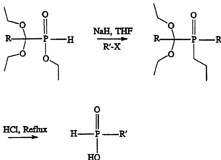
SCHEME I
