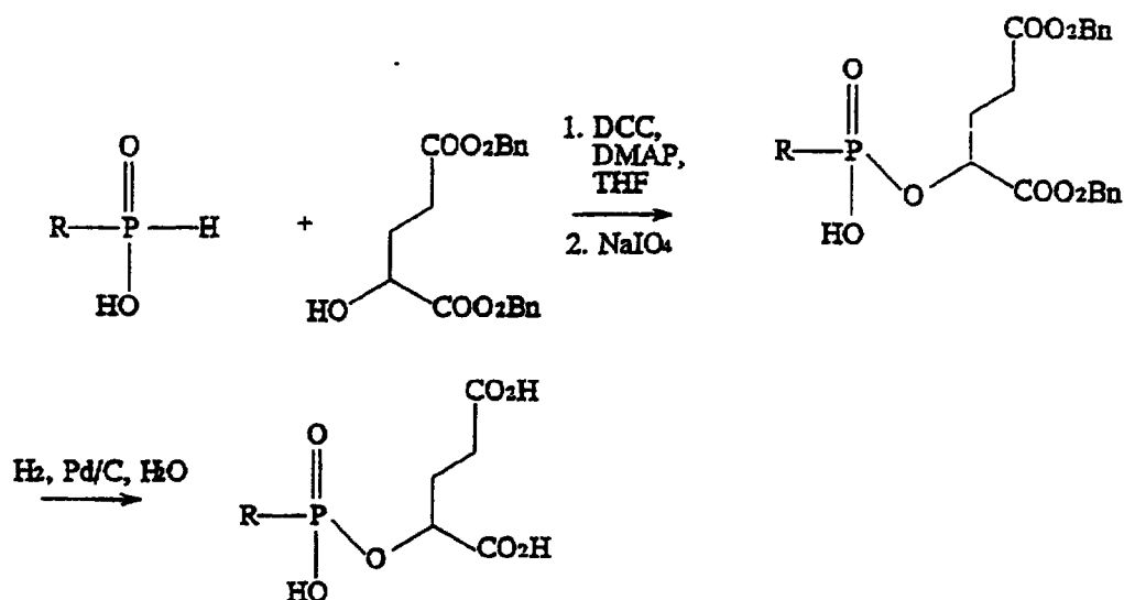
SCHEME IX
