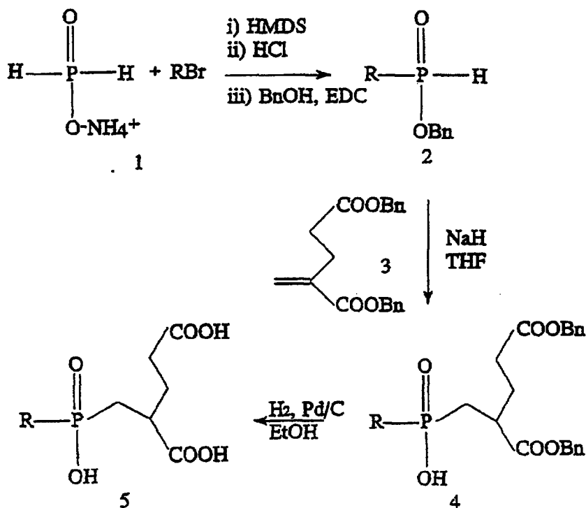
SCHEME V
