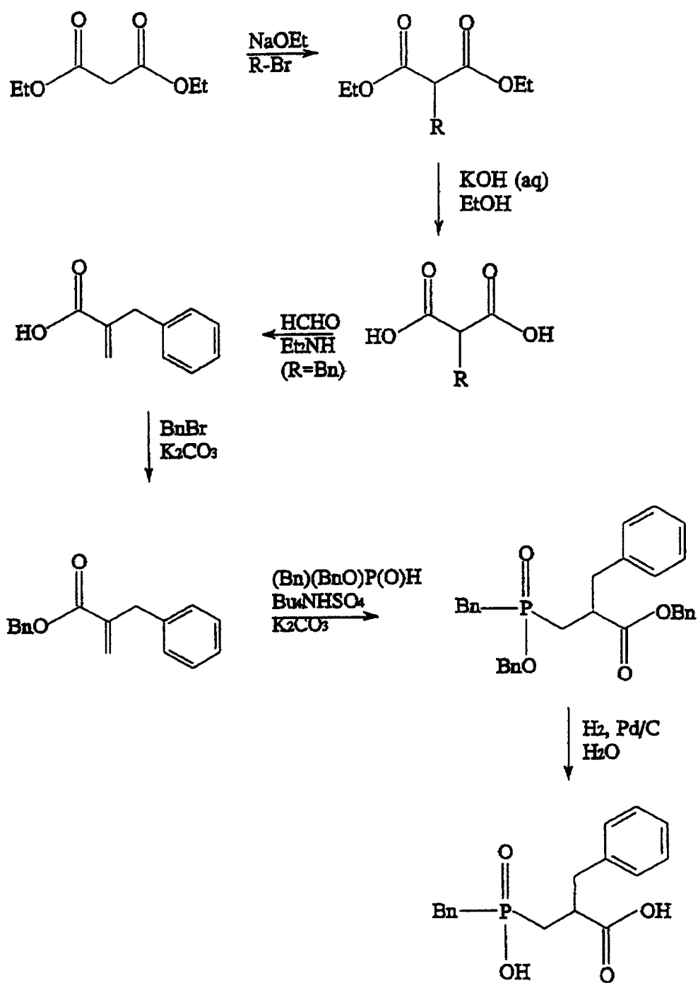
SCHEME VII
