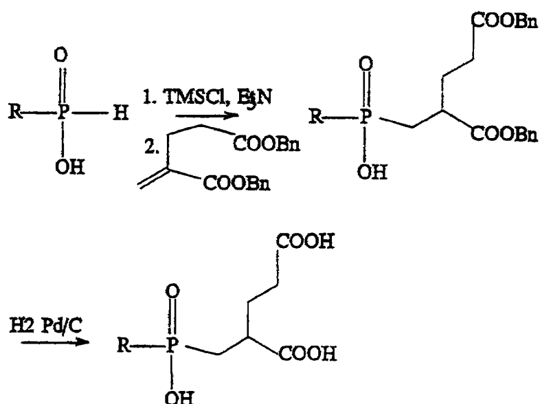
SCHEME III
