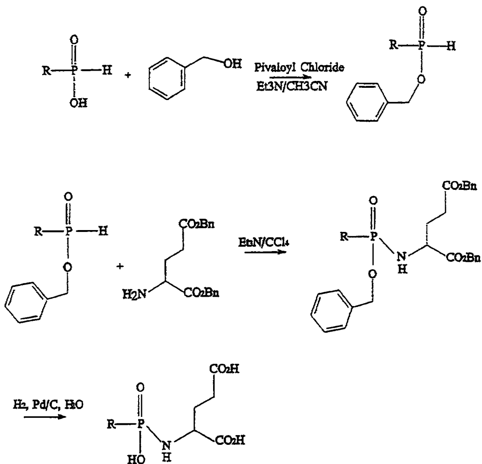
SCHEME VIII
