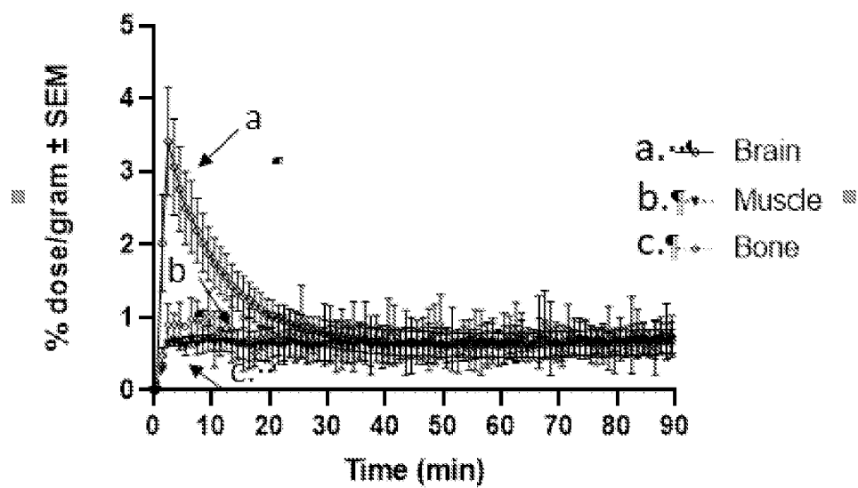
Figure 1B. 90 minute PET time activity curves for [ ^{18}\text{F} ]-N-(4-(1,2,4,5-tetrazin-3-yl)benzyl)-4-fluorobenzamide (Brain, Muscle, & Bone, N=2)
