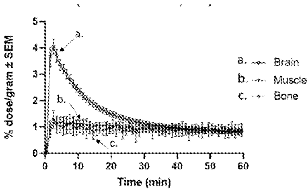
Figure 1A. 60 minute PET time activity curves for [ ^{18}\text{F} ]-N-(4-(1,2,4,5-tetrazin-3-yl)benzyl)-4-fluorobenzamide (Brain, Muscle, & Bone, N=4)
