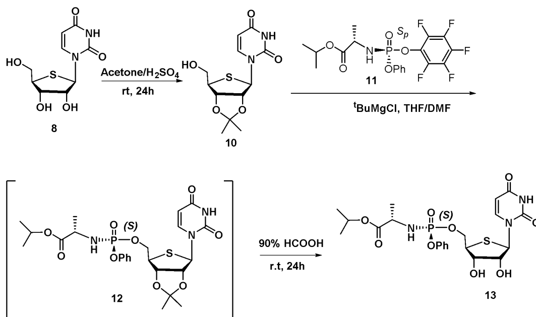
Scheme 3: Synthesis of compound 13
