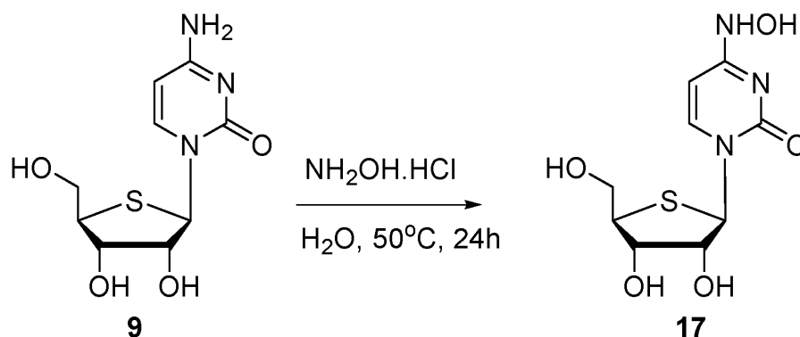
Scheme 5: Synthesis of compound 17
