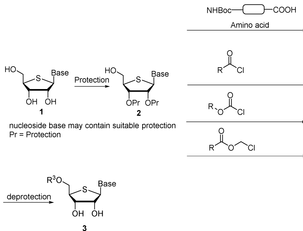
Scheme 1: A synthetic approach to nucleosides 3 .
