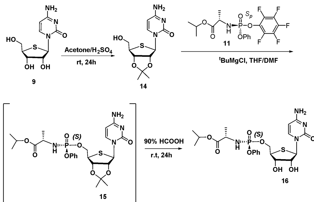
Scheme 4: Synthesis of compound 16
