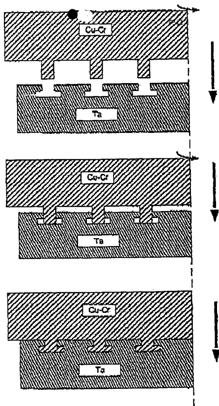
Friction weld interlocking target assembly method.
