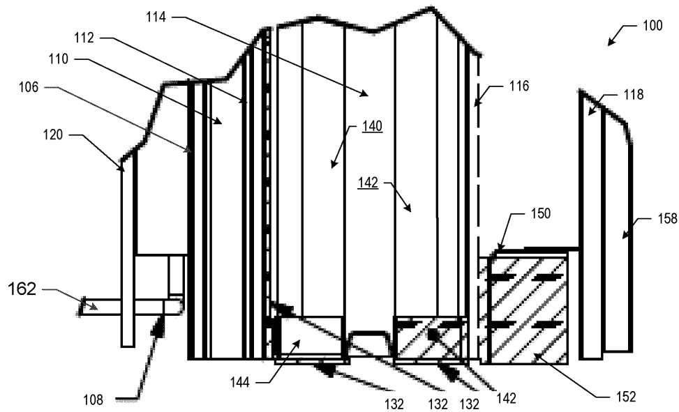
DETAIL C FIG. 5
