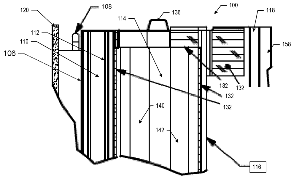
DETAIL D FIG. 6
