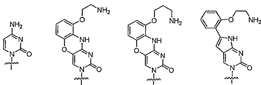
Cytosine and Modified Cytosines
