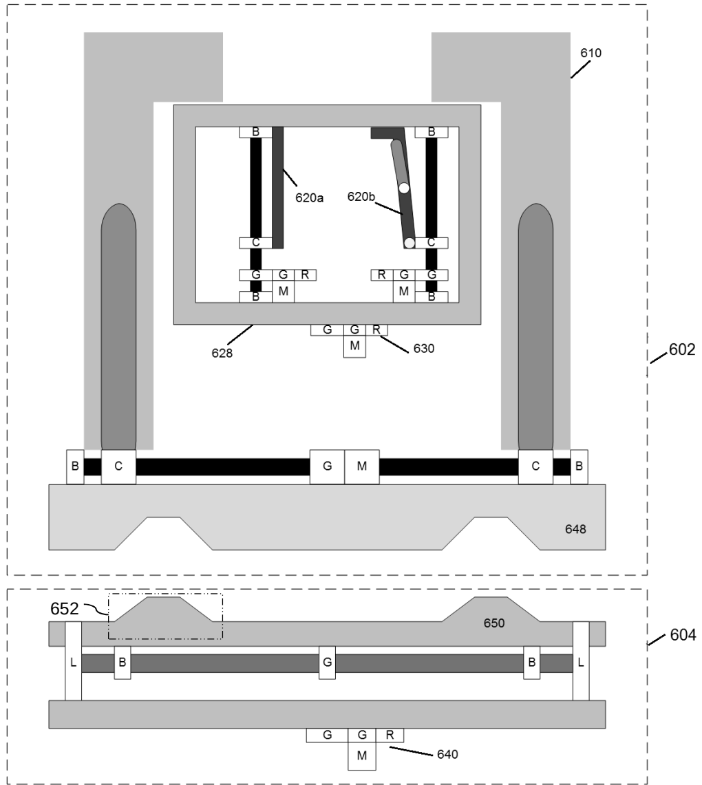
Side view of End effector
