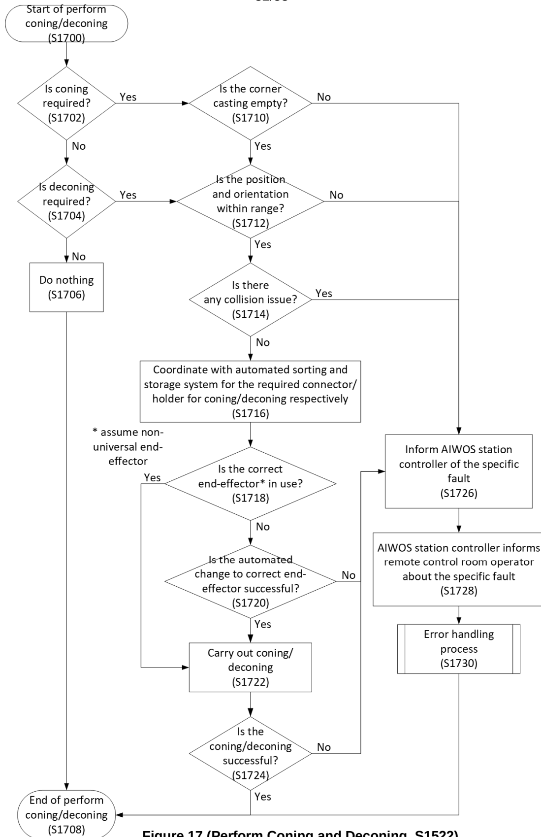
Figure 17 (Perform Coning and Deconing, S1522)
