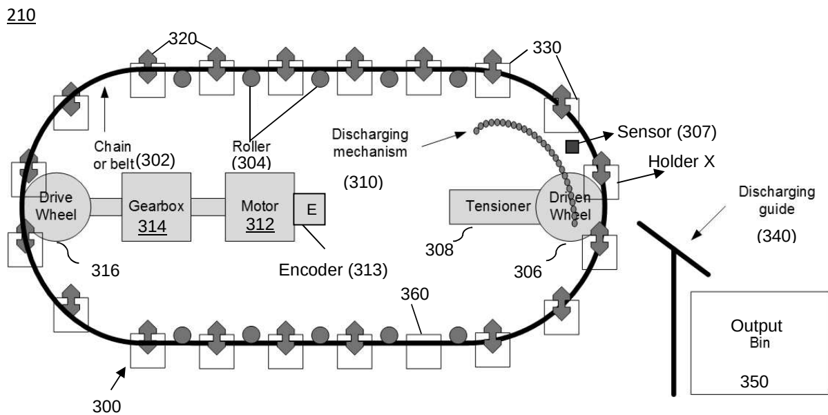
Figure 3A (Side View)
