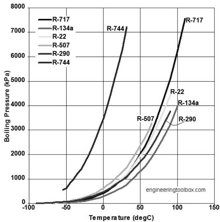
Refrigerant pressure vs temperature chart.
