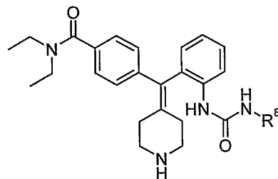
Compound 10: R^8 = Ph Compound 22: R^8 = CH_2Ph
