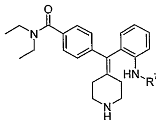
Compound 9: R^7 = C_6H_{11} Compound 20: R^7 = C_6H_9 Compound 21: R^7 = C_7H_{13}
