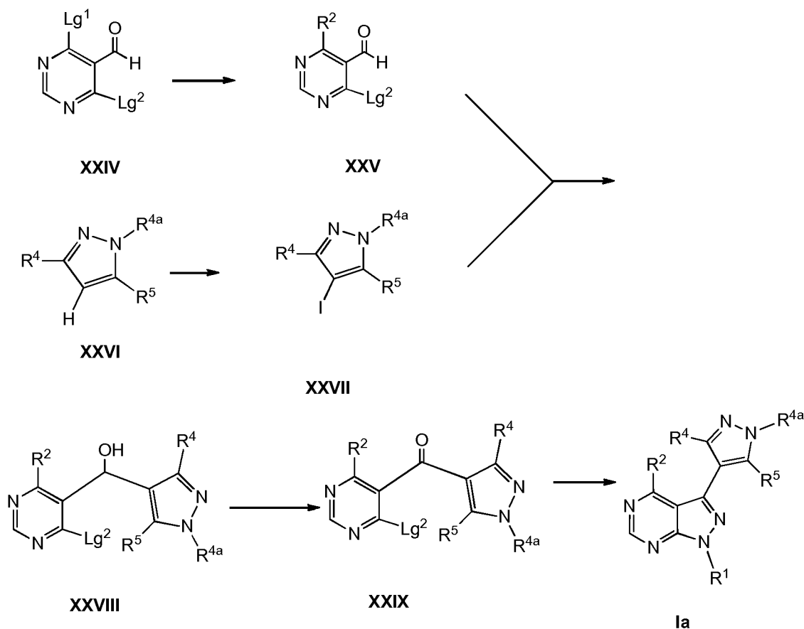
Scheme 11
