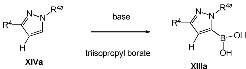
Scheme 8
