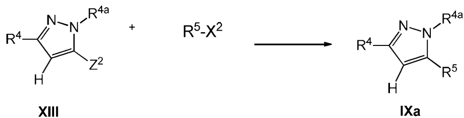
Scheme 7
