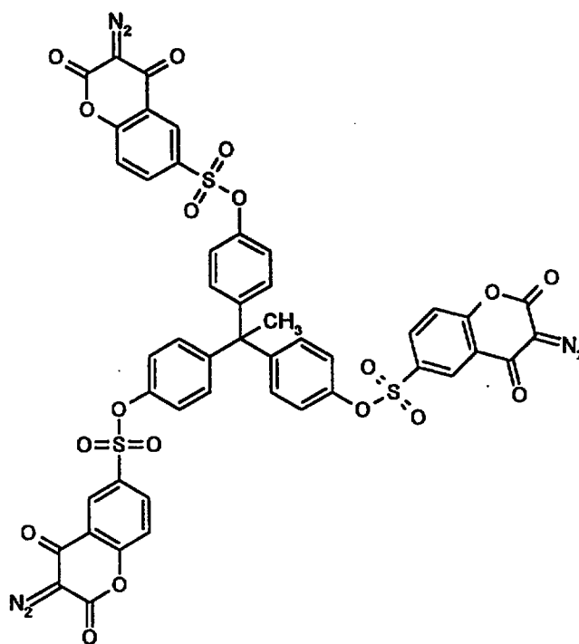
4,4'-bis(3-diazo-4-oxo-3,4-dihydrocoumarin-6-sulfonyloxy)benzophenone
