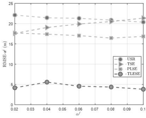
(a) Position estimation error
