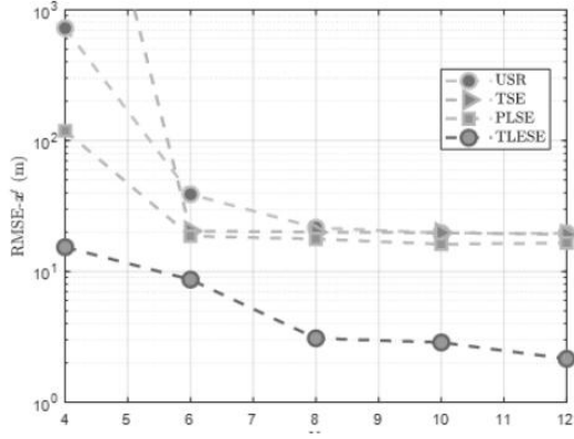
(a) Position estimation error
