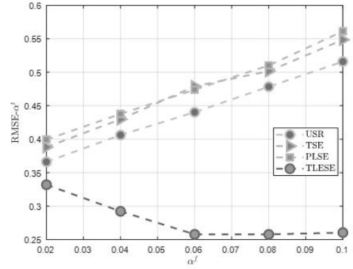
(b) Path loss factor estimation error
