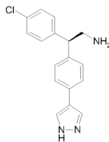
Isomer D
