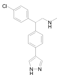
Isomer A
