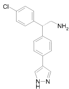
Isomer C
