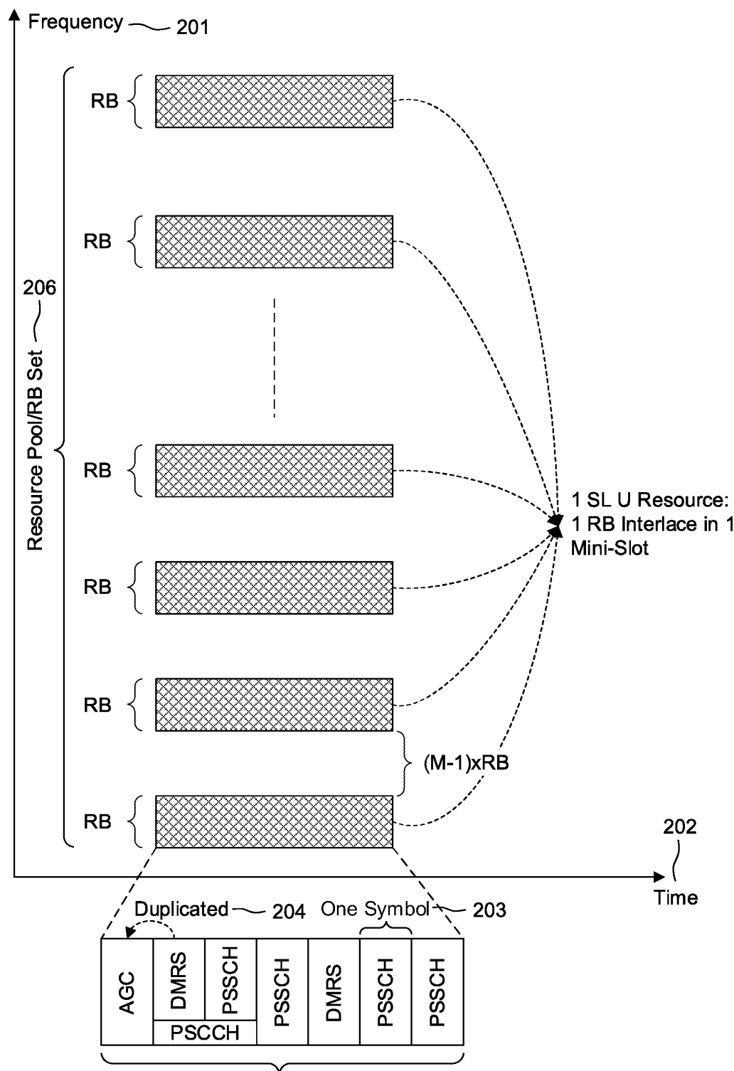
A Mini-Slot for PSCCH/PSSCH Transmission with 7 Symbols Including 1 AGC Symbol at the Beginning of the Slot — 205B
