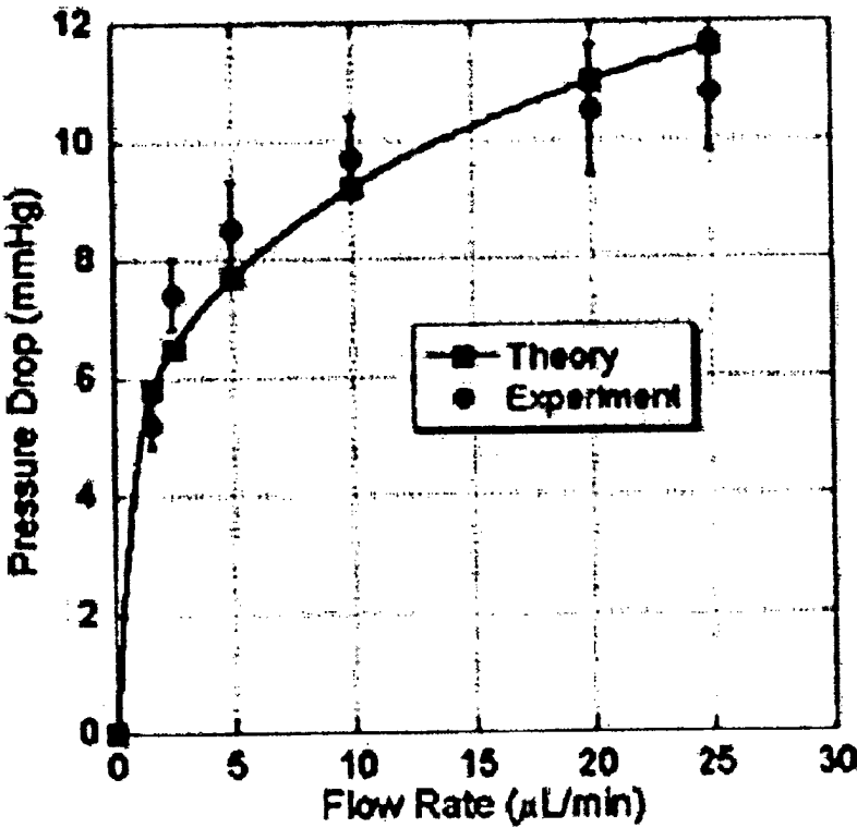
FIG. 4 (Prior art)
