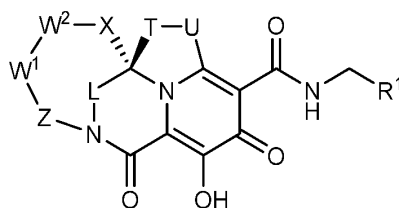
Formula IIa.
