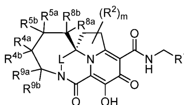
Formula VIb;
