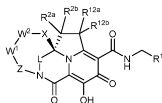
Formula IVb.
