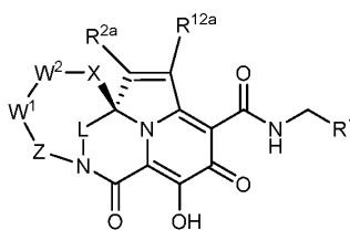
Formula Vb.
