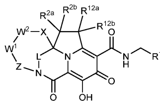
Formula IV.
