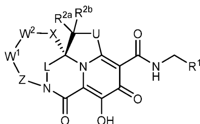
Formula IIIa.
