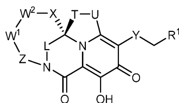
Formula Ia.
