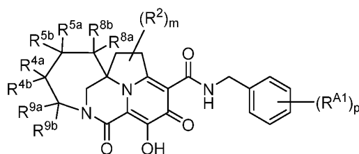
Formula VIII;
