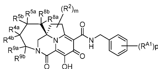
Formula VIIIb;
