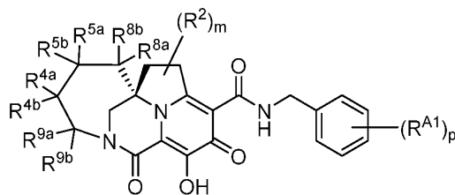
Formula VIIIa;
