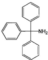
Triphenylmethanimine
