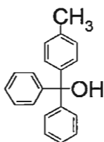
(Compound 24)
