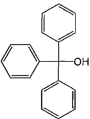
Triphenylmethanol
