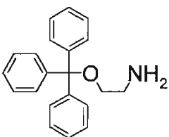
2-(Triphenylmethyloxy)ethylamine (Compound 4)
