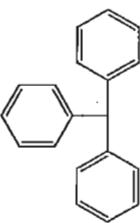
Triphenylmethane
