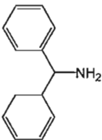
Aminodiphenylmethane
