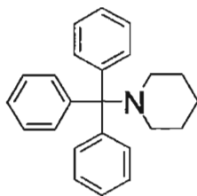
1-(Triphenylmethyl)piperidine (Compound 5)
