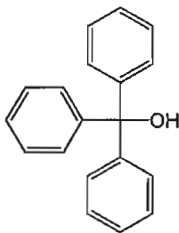
Triphenylmethanol
