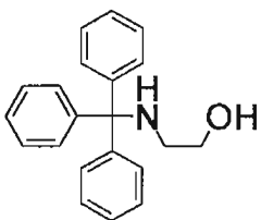
2-(Triphenylmethylanino)ethanol (Compound 3)
