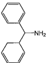
Aminodiphenylmethane
