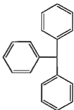
Triphenylmethane
