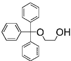
2-(Triphenylmethyloxy)ethanol (Compound 2)
