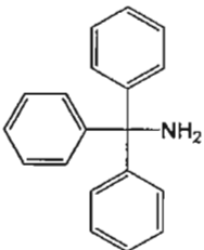
Triphenylmethylanine
