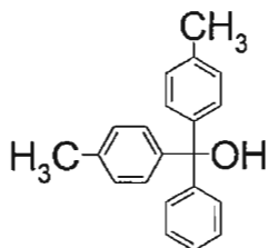
(Compound 23)
