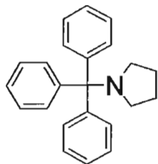
1-(Triphenylmethyl)piperidine (Compound 5)
