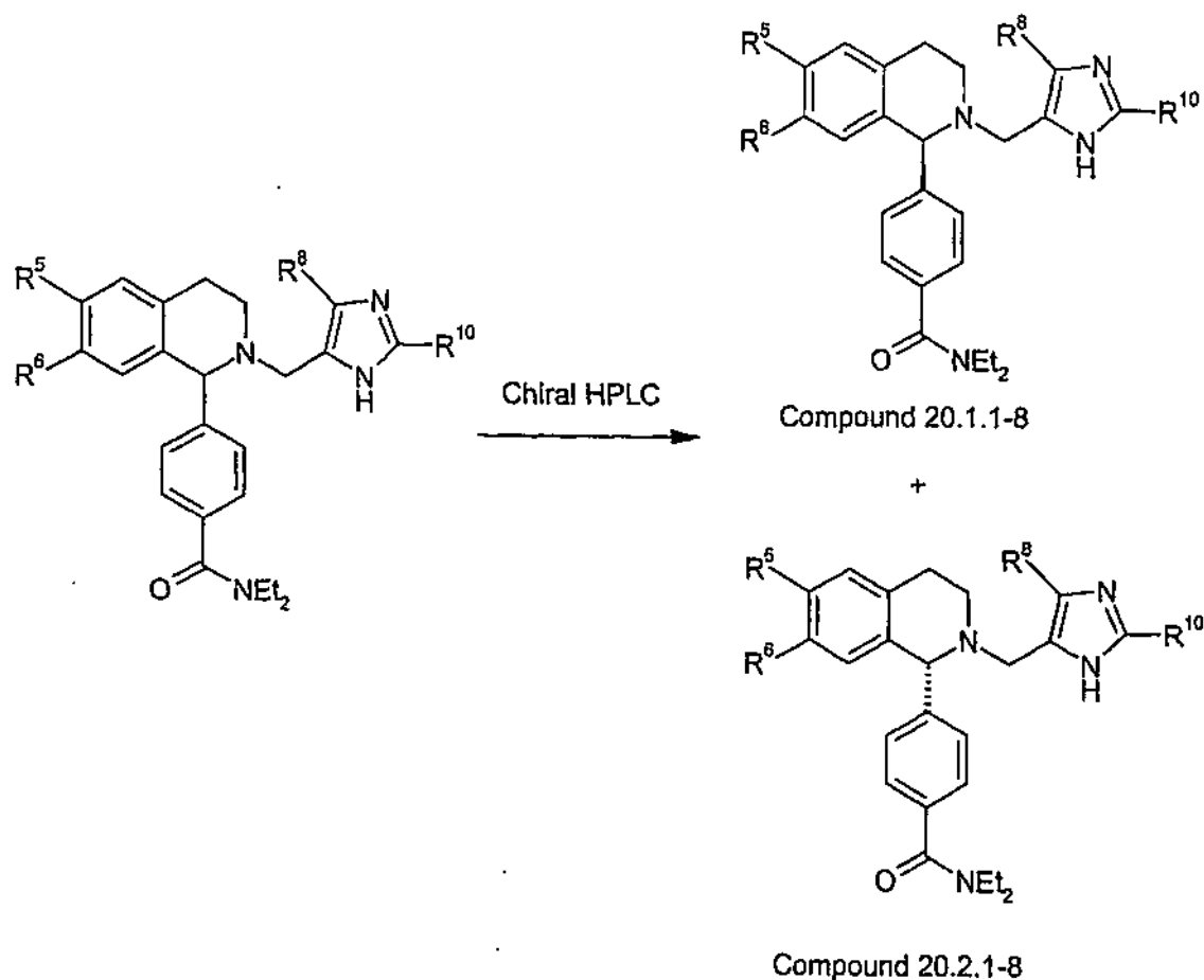
Scheme 20
