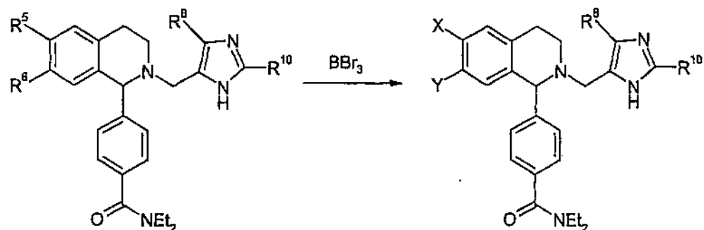
Compound 12.1.9-11, 21, 44, 14.1.1-4
