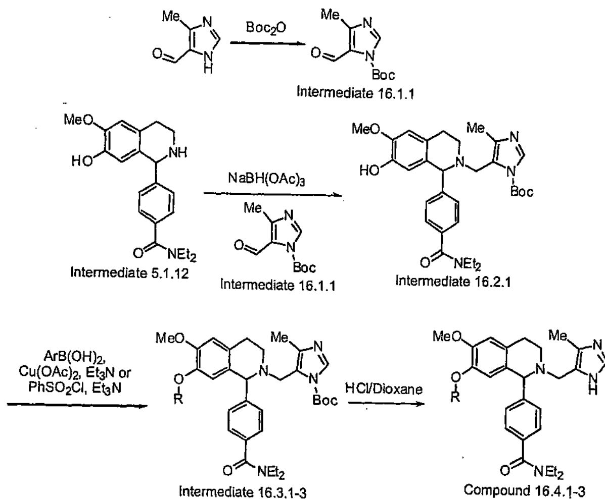
Scheme 16
