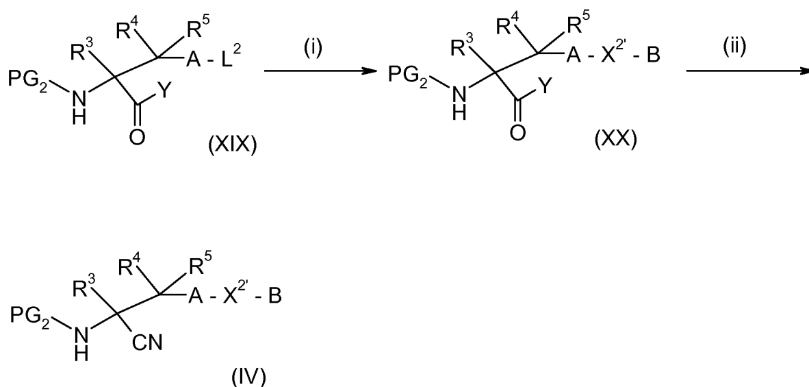
Reaction Scheme 1
