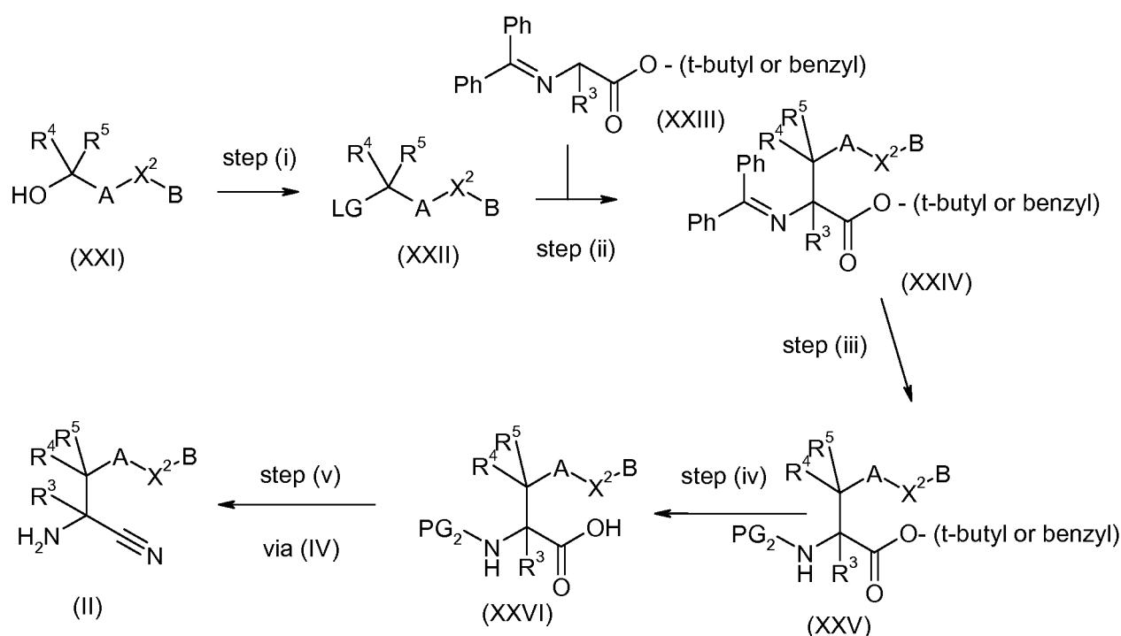
Reaction Scheme 2
